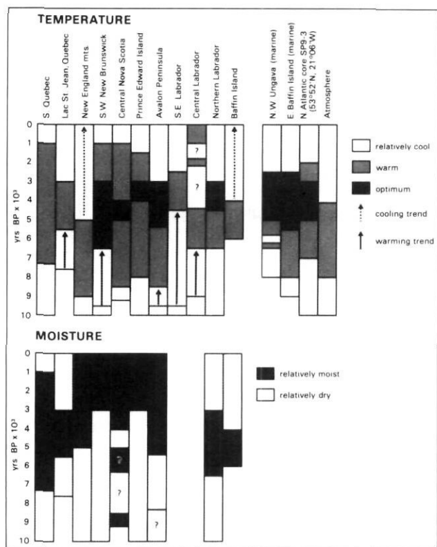
FIGURE 9. Inferred Holocene climatic conditions, northeastern North America. Sources: S. Québec and Lac Saint-Jean: RICHARD (1978, 1980a); New England mountains: DAVIS et al. (1980); S.W. New Brunswick: MOTT (1975a); Central Nova Scotia: HADDEN (1975); Prince Edward Island: ANDERSON (1980); Avalon Peninsula: author; S.E. Labrador: LAMB (1980); Central Labrador: JORDAN (1975); N. Labrador: SHORT (1978); Baffin Island: ANDREWS et al. (1980); N.W. Ungava (marine) and E. Baffin Island (marine): ANDREWS (1972); N. Atlantic core SP9-3: WOLLIN et al. (1971); Atmosphere: DANSGAARD et al. (1971).
