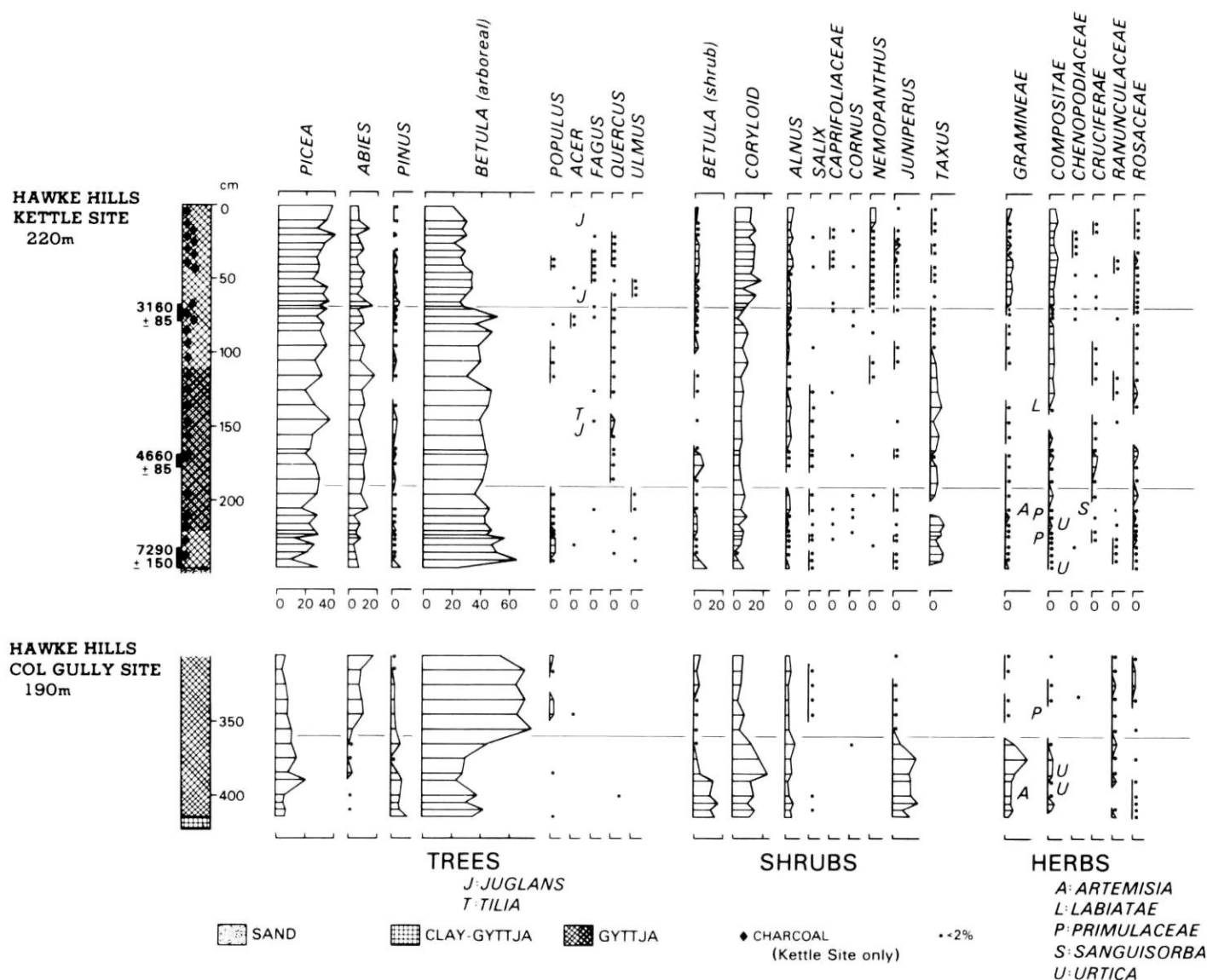
FIGURE 7. Pollen diagrams, Hawke Hills kettle and col gully sites.
