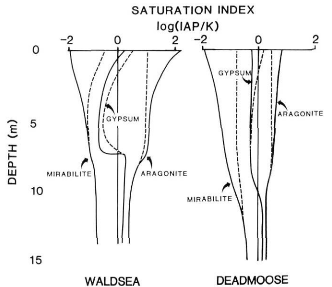
FIGURE 4. Degree of saturation with respect to aragonite, gypsum, and mirabilite of Waldsea and Deadmoose lakes. Solid lines are for summer; dashed lines are for winter. Saturation indices calculated using WATSPEC (WIGLEY, 1977).
