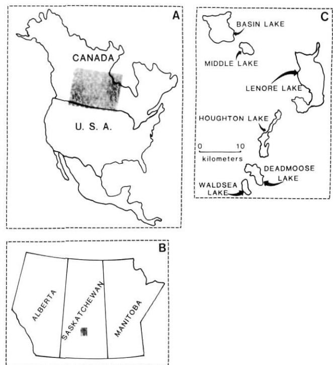
FIGURE 1. Maps showing the location of Waldsea and Deadmoose lakes in the Northern Great Plains of North America. North is toward the top on all the figures.
