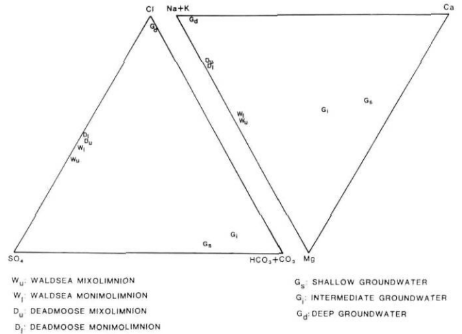
FIGURE 3. Ternary diagram showing average ionic composition (in percent equivalents) of water from Waldsea and Deadmoose lakes and groundwater of the area.
