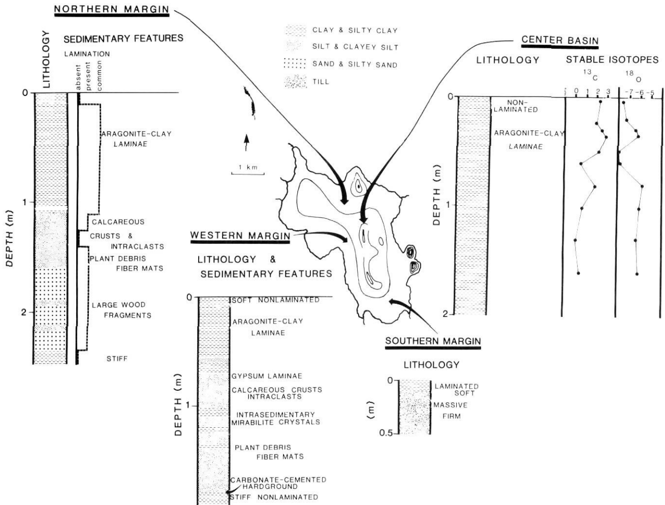
FIGURE 7. Representative stratigraphic sequences from Deadmoose Lake. Contour interval on the bathymetric map is 10 m. Stable isotope values are reported in \delta\% PDB for carbon and \delta\% SMOW for oxygen.
