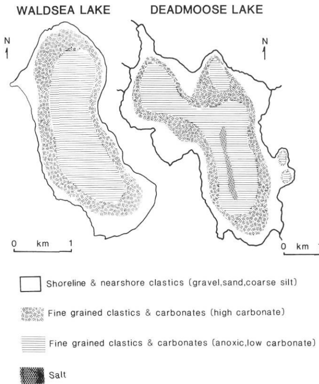
FIGURE 5. Modern sediment distribution in Waldsea and Deadmoose lakes.
