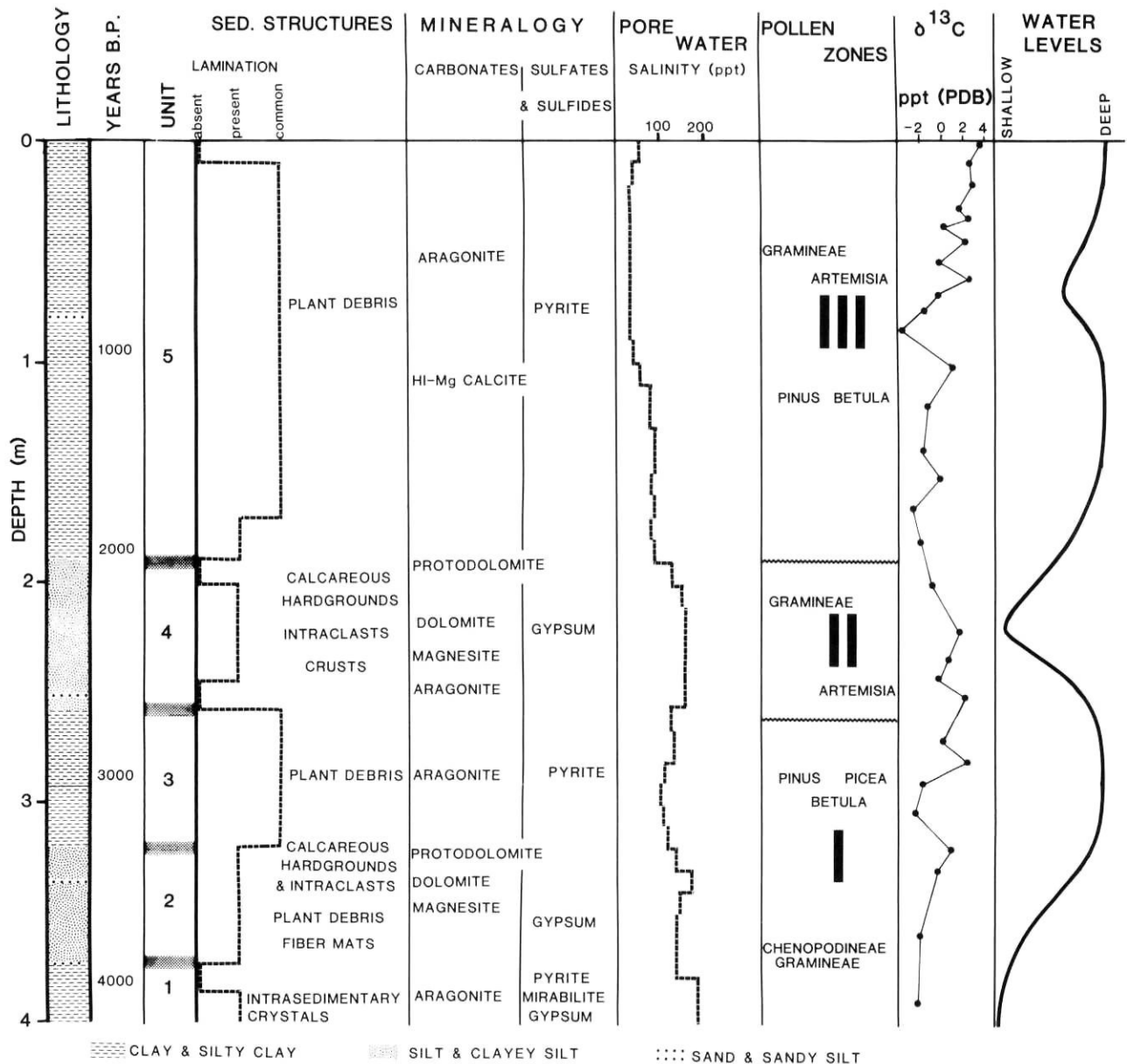
FIGURE 6. Summary of Waldsea Lake stratigraphy. Pore water salinity is reported in parts per thousand (ppt). The lithologic sequence, radiocarbon chronology, sedimentary structures, and mineralogy represent syntheses of information from all the cores in the basin. The pore water salinity, pollen stratigraphy, and stable isotope values are derived from single cores. The water level curve is an interpretation based mainly on the lithostratigraphy.
