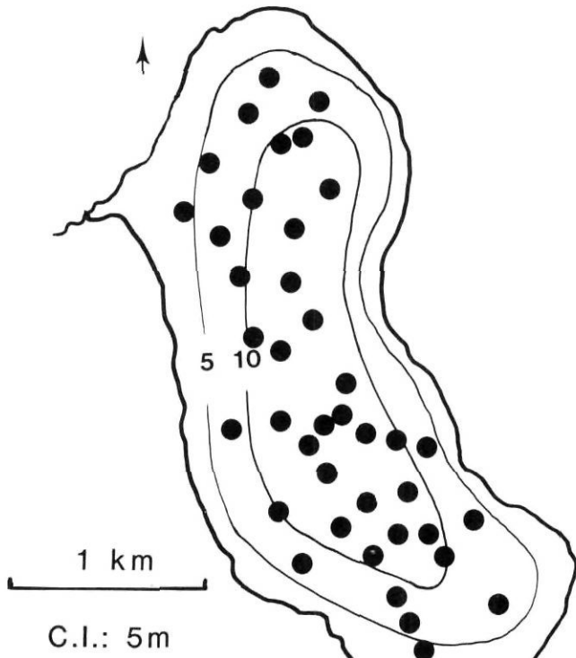
FIGURE 2. Bathymetric contour maps of Waldsea and Deadmoose lakes. Black dots indicate core locations. The X's in Deadmoose Lake indicate holes greater than 45 m in depth.
