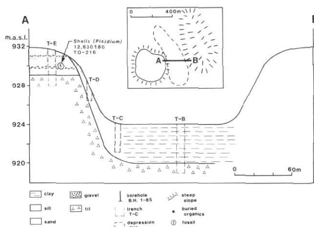
FIGURE 27. Photo (ISPG 2482-26) of the Ham Site viewed north-east from the margin of a moraine plateau (foreground) across a depression in hummocky dead-ice moraine of the Boundary Plateau. Stratigraphic cross-section of the Ham Site located in NW 1/4 sec. 28, tp. 1, rge. 21 (49°04'05"N, 108°45'30"W). Radiocarbon date listed in Table I.
