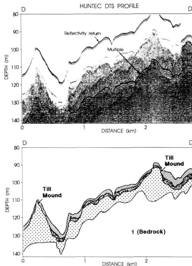
FIGURE 7. Seismic profile D-D' (Fig. 1), showing mounds formed by unit 2. Unit 3 onlaps each side of the ridges and is absent on their crests (Figure 4 for legend).
