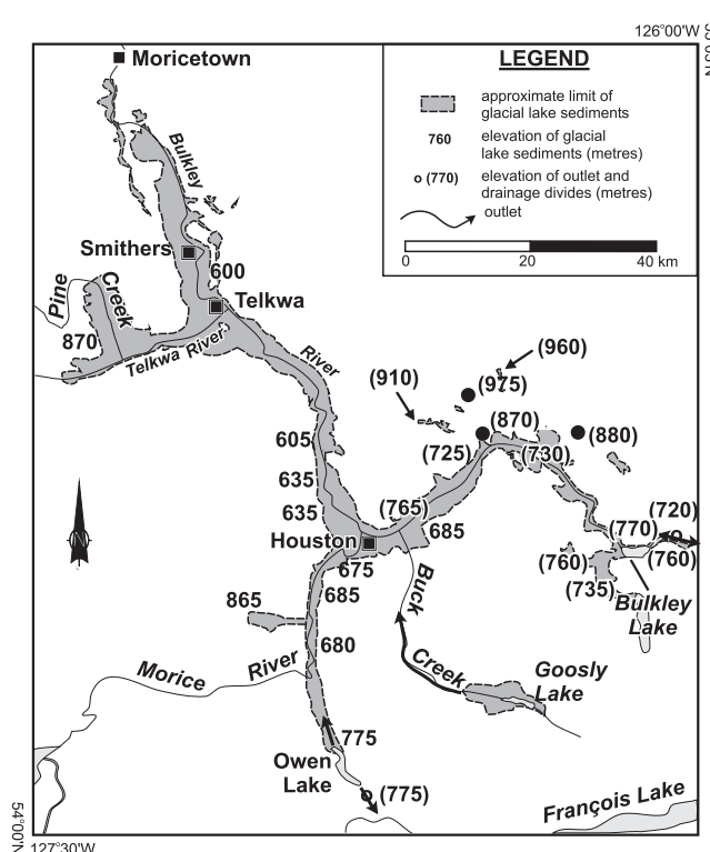
FIGURE 9. The maximum elevation of late-glacial glaciolacustrine sediments in the Bulkley River region. The limits of these proglacial lakes were defined using field data, interpretations of the surficial geology from 1:60 000- to 1:70 000-scale aerial photographs, and observations and data by Farstad and Laird (1954), Runka (1972), Clague (1984), and Church and Barakso (1990).
