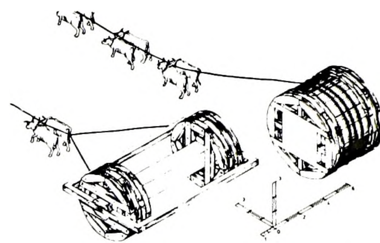
FIGURE 1. Isometric restorations of machines used in the transport of colossal stones. From Coulton.
