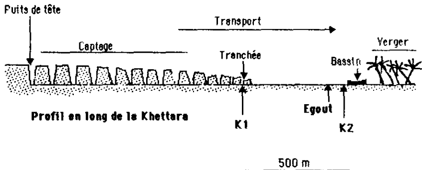
Figure 1 Descriptions of a khattara system. Drainage of the aquifer by a khattara.
