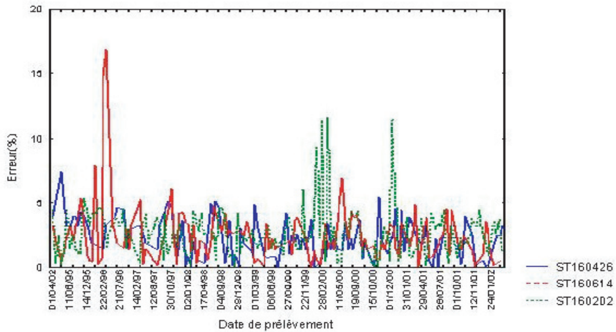
Figure 1 Balance ionique. Ion balance.
