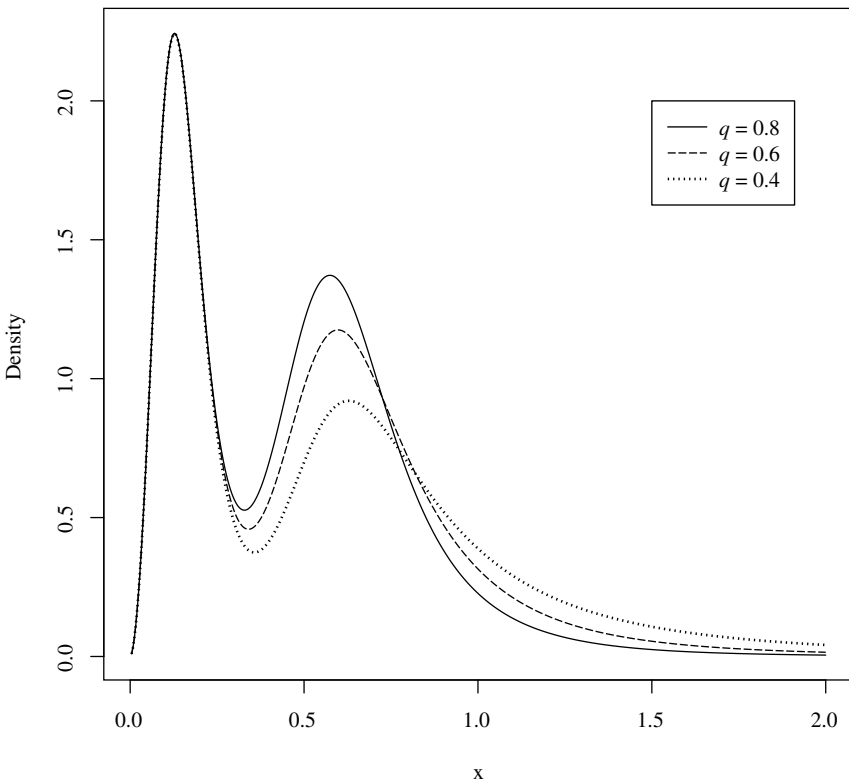
FIGURE 1 MIXTURE OF TWO SINGH-MADDALA DISTRIBUTIONS
