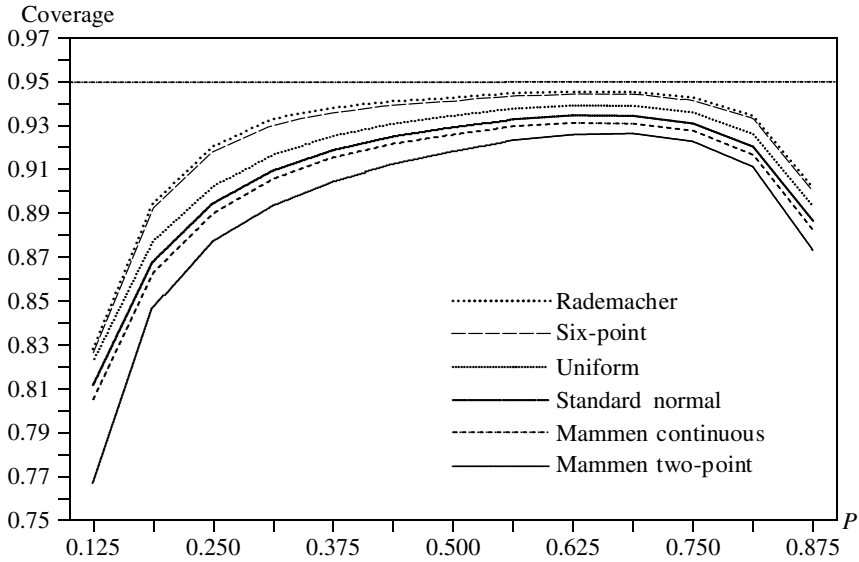
FIGURE 7 COVERAGE OF STUDENTIZED BOOTSTRAP INTERVALS VERSUS P FOR G = 16, \gamma = 3, \pi = 0.4
