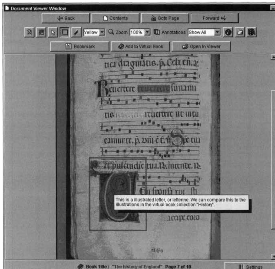
Figure 3 : Annotations (DEBORA)
