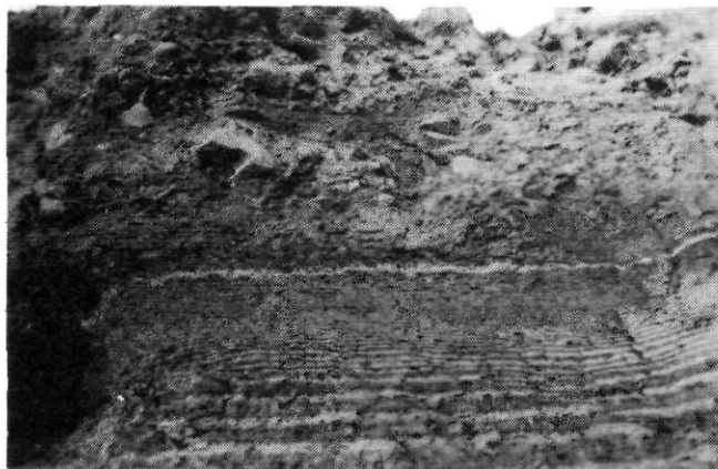
FIGURE 13. Upward thinning rhythmically bedded glaciomarine sediment at top of Section 1 overlain by 0.5 m of till, both facies of Unit 5; freshly cleaned damp face (cf. Fig. 17) (GSC-203537-U).
