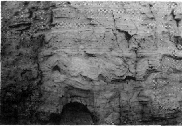
FIGURE 16. Convolute lamination in the middle zone of the stratified glaciomarine diamicton facies of Unit 5 at top of Section 1; note abundant dropstones. Trowel blade is about 8 cm wide (GSC-203537-W).
