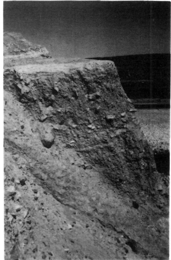
FIGURE 5. Top 6 m or so of thick diamicton at base of Section 5. Slight horizontal stratification produced by thin sand/silt laminae between till-like beds. Diamicton is capped by rhythmically bedded, plane laminated fine sand and silt (distal glaciomarine sediment) (GSC-203536-Z).
