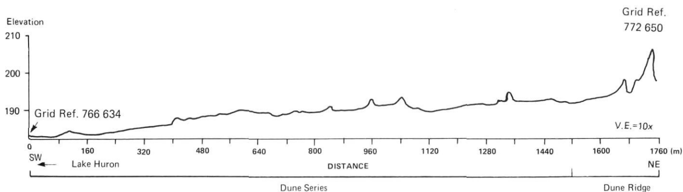
FIGURE 3. Transect across the dune field from the eastern dune ridge to the modern shoreline at Howdenville Bay.
