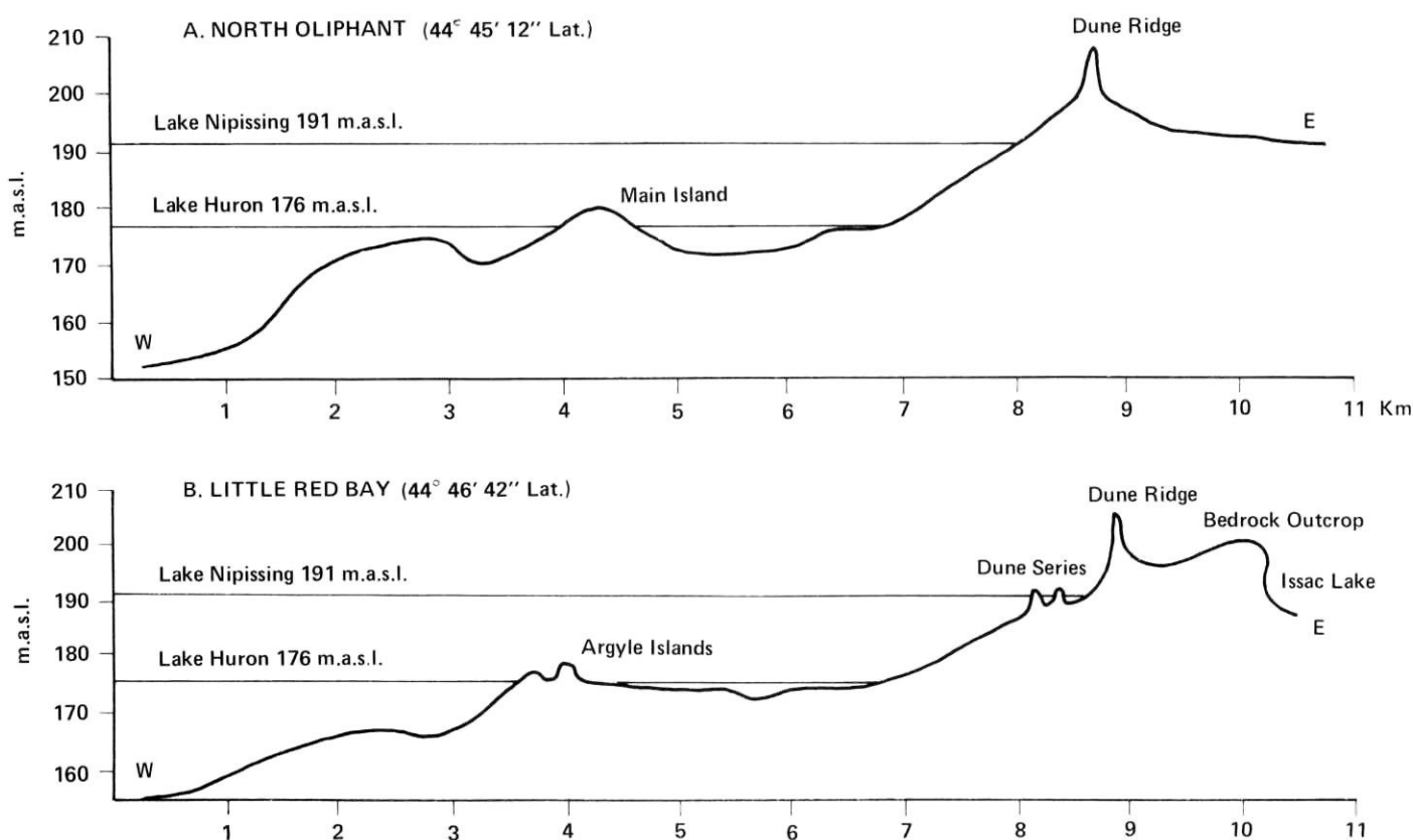
FIGURE 5. Profiles across the dune field and nearshore at two locations, illustrating the effects of lake level changes on shoreline exposure. The profiles are based on the 1:50,000 topographic map and 1:75,000 hydrographic chart of the area.
