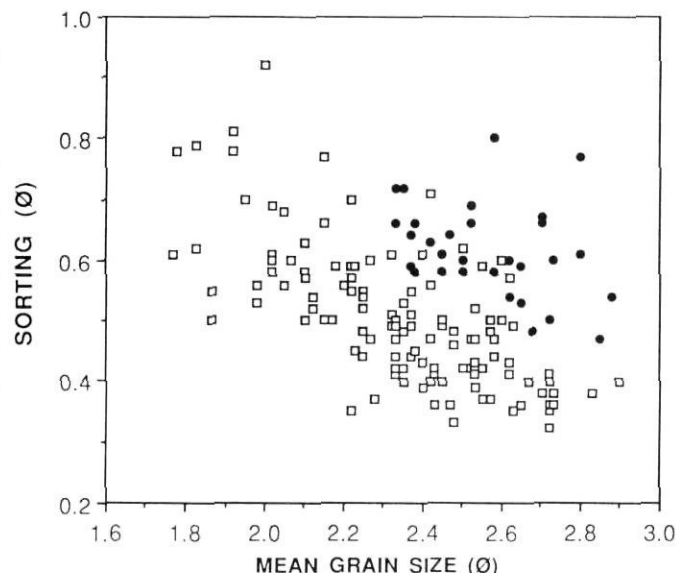
FIGURE 5. Mean grain size and sorting from parabolic and dome dunes in the Grande Prairie Dune Field. Circles represent dome dunes. Squares represent parabolic dunes. Sediments of assemblage G are excluded. Sorting values calculated according to Folk and Ward (1957).
