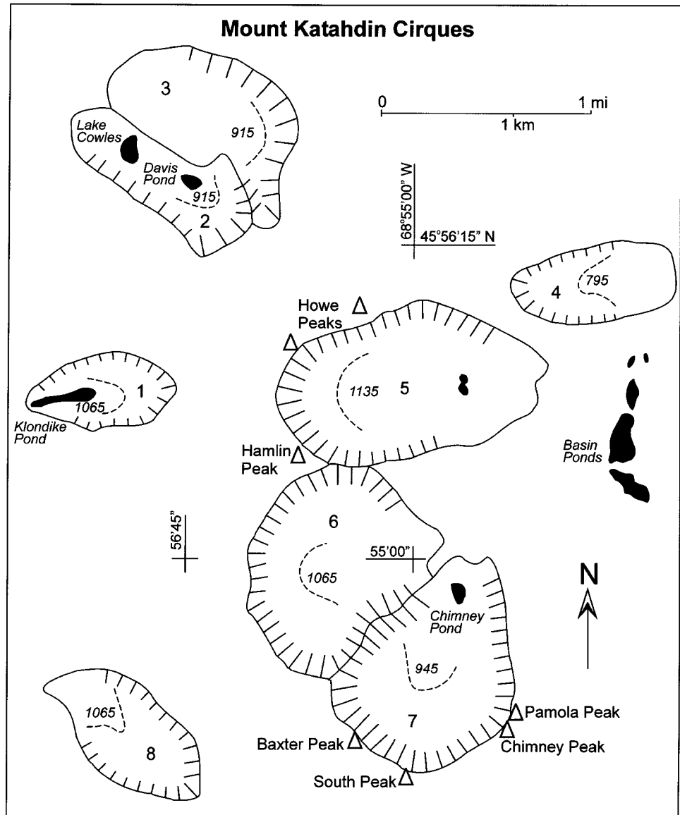
FIGURE 5. Cirque morphometric map for Mount Katahdin, Maine. Solid lines indicate outlines of cirques, hachured solid lines are cirque headwalls, dashed lines are cirque schrunds, with altitudes indicated in meters. Cirque numbers refer to Table I. Water bodies shown in black for cirques #1, 2, 5, and 7, and along Basin Ponds moraine east of cirques #5, 6, and 7.
