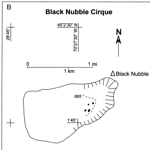
FIGURE 6. A. Cirque morphometric maps for Longfellow Mountains, Maine. Solid lines indicate outlines of cirques, hachured solid lines are cirque headwalls, dashed lines are cirque schruns, with altitudes indicated in meters. Numbers for cirques on Sugarloaf and Crocker Mountains refer to Table I; only cirque #6 has small water body, shown in black. B. Black Nubble cirque; water bodies shown in black.
