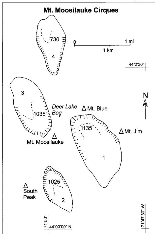
FIGURE 4. Cirque morphometric map for Mount Moosilauke. Solid lines indicate outlines of cirques, hachured solid lines are cirque headwalls, dashed lines are cirque schunds, with altitudes indicated in meters. Numbers refer to Table I.
