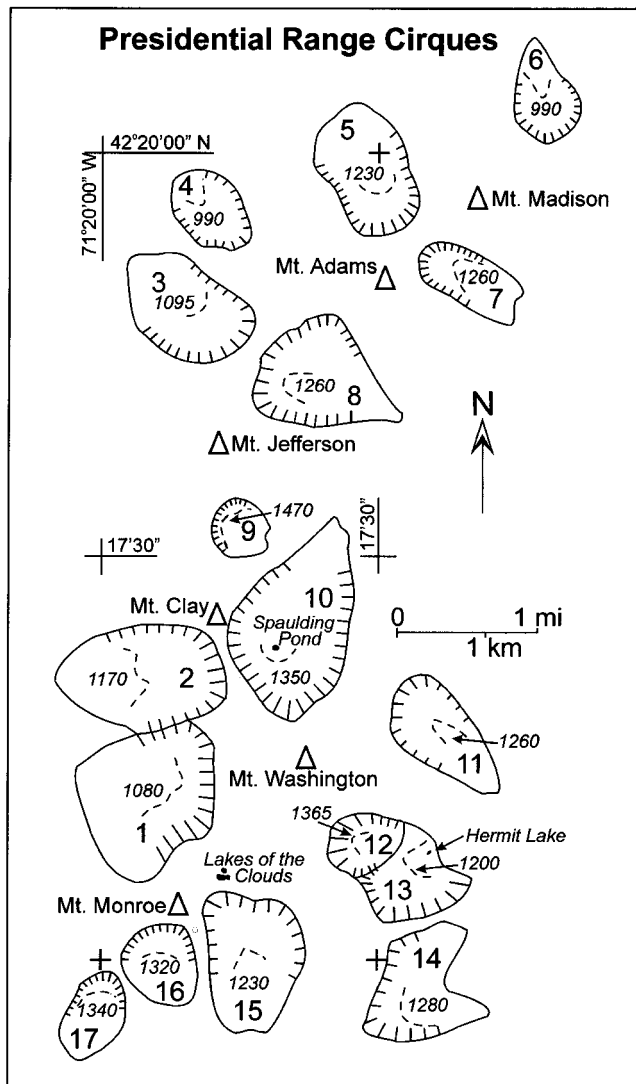
FIGURE 3. Cirque morphometric map for Presidential Range. Solid lines indicate outlines of cirques, hachured solid lines are cirque headwalls, dashed lines are cirque schruns, with altitudes indicated in meters. Numbers refer to Table I. Small water bodies shown in black for cirques #10 and 13.
