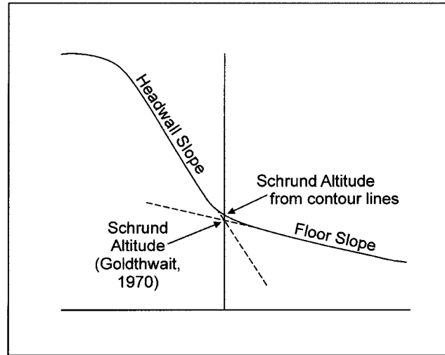
FIGURE 2. Schematic illustration for estimation of schrund altitude (after Goldthwait, 1970, Fig. 9, p.100).
