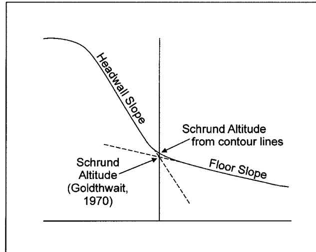
FIGURE 2. Schematic illustration for estimation of schrund altitude (after Goldthwait, 1970, Fig. 9, p.100).
