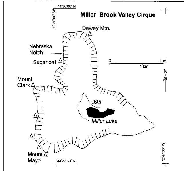
FIGURE 7. Cirque morphometric map for Miller Brook valley cirque, Green Mountains, Vermont. Solid line indicates outline of cirque, hachured solid line is cirque headwall, dashed line is cirque schrand, with altitude indicated in meters. Miller Lake is labeled.
