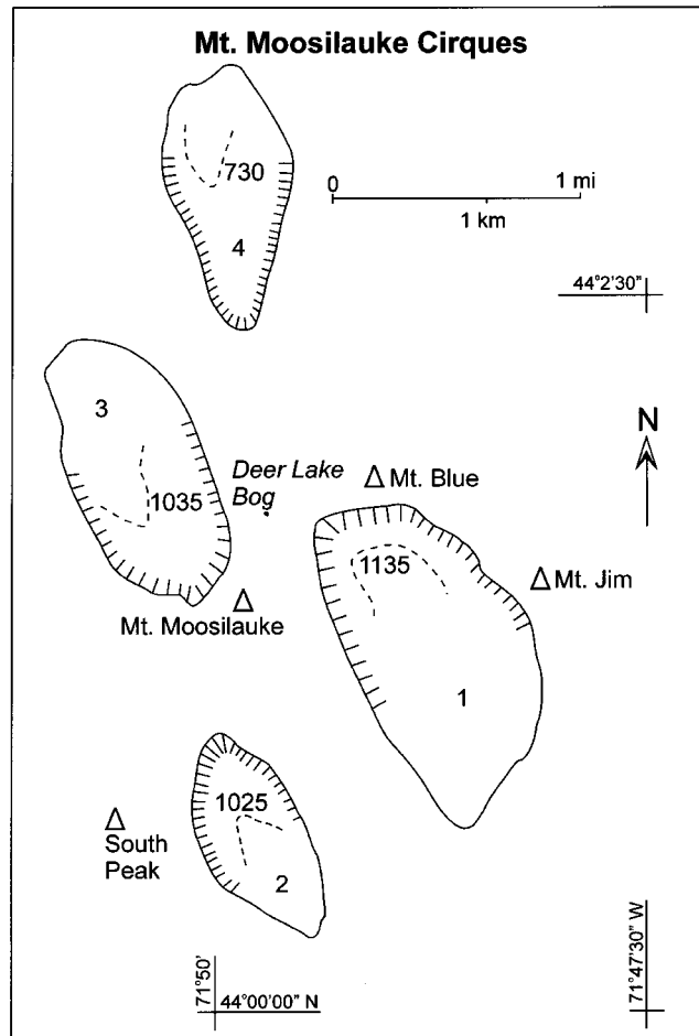
FIGURE 4. Cirque morphometric map for Mount Moosilauke. Solid lines indicate outlines of cirques, hachured solid lines are cirque headwalls, dashed lines are cirque schtrunds, with altitudes indicated in meters. Numbers refer to Table I.
