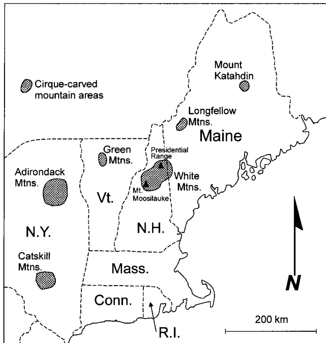
FIGURE 1. Index map for alpine areas with cirques in northeastern United States (after Bradley, 1981, and Ackerly, 1989).
