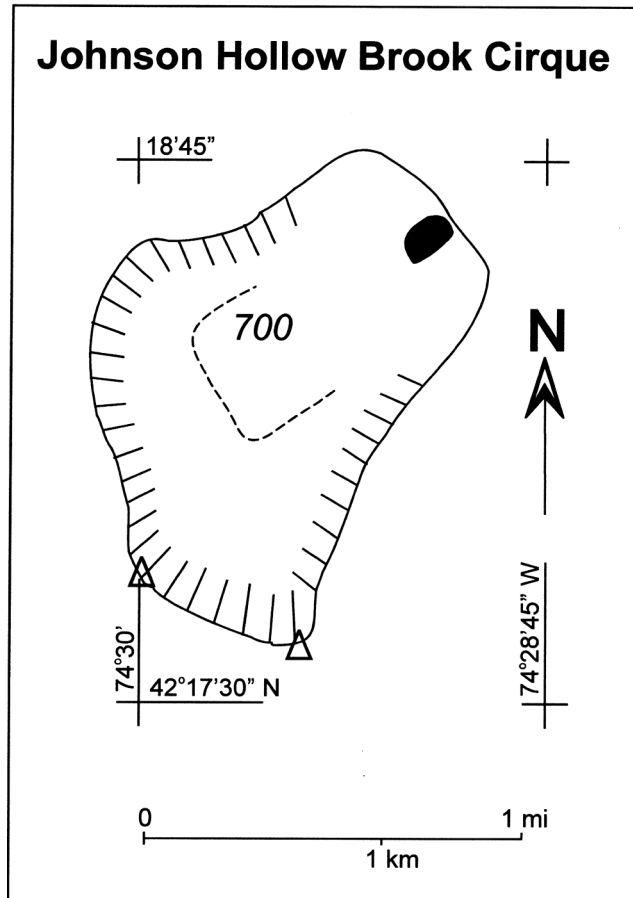
FIGURE 11. Cirque morphometric map for Johnson Hollow Brook, Catskill Mountains, New York. Solid line indicates outline of cirque, hachured solid line is cirque headwall, dashed line is cirque schrand, with altitude indicated in meters. Water body shown in black.
