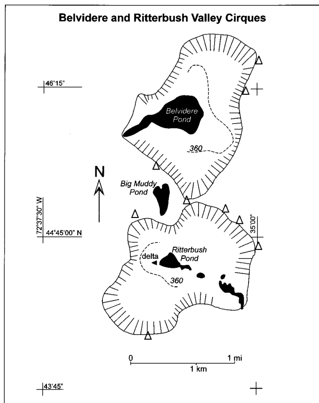
FIGURE 8. Cirque morphometric map for Belvidere (north) and Ritterbush valley (south) cirques, Green Mountains, Vermont. Solid lines indicate outlines of cirques, hachured solid lines are cirque headwalls, dashed lines are cirque schrunds, with altitudes indicated in meters. Water bodies shown in black, except for Belvidere and Ritterbush ponds, which are labeled.
