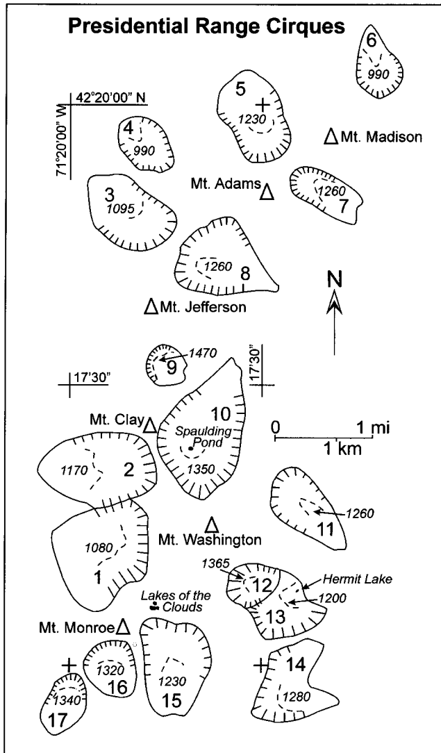
FIGURE 3. Cirque morphometric map for Presidential Range. Solid lines indicate outlines of cirques, hachured solid lines are cirque headwalls, dashed lines are cirque schrunnds, with altitudes indicated in meters. Numbers refer to Table I. Small water bodies shown in black for cirques #10 and 13.
