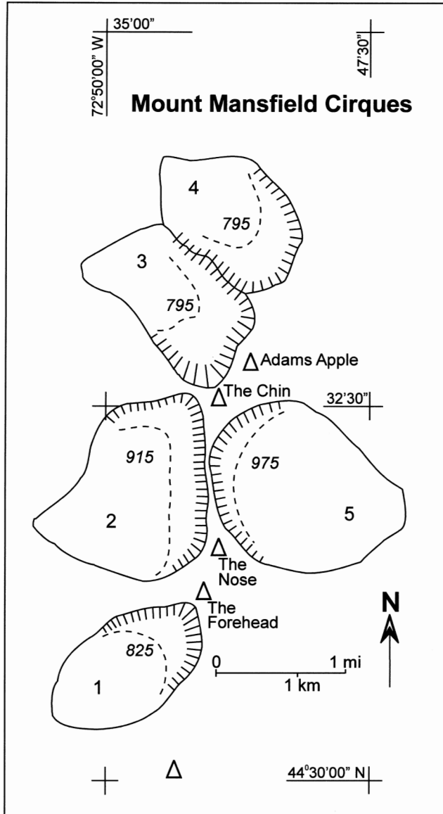
FIGURE 9. Cirque morphometric map for Mount Mansfield, Vermont. Solid lines indicate outlines of cirques, hachured solid lines are cirque headwalls, dashed lines are cirque schrunds, with altitudes indicated in meters. Cirque numbers refer to Table I.
