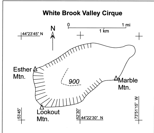
FIGURE 10. Cirque morphometric map for White Brook valley, Adirondack Mountains, New York. Solid line indicates outline of cirque, hachured solid line is cirque headwall, dashed line is cirque schrund, with altitude indicated in meters.
