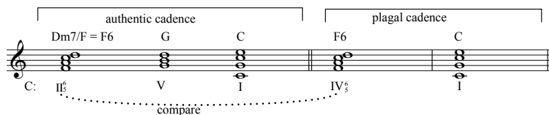
Example 4 II 6 6 and IV 6 6 contain the same notes. IV is used when the chord moves directly to the tonic (plagal cadence).
