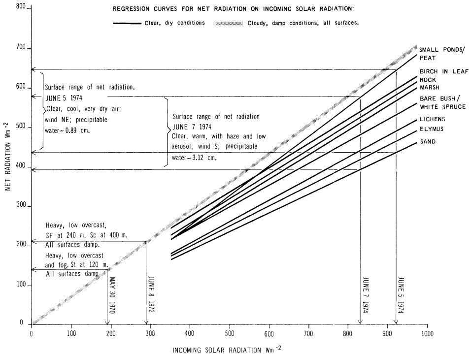
POSTE - DE - LA - BALEINE : Range of global and net radiation fluxes (horizontal surface) for clear, dry weather and damp, cloudy conditions. Some extreme noon values.
