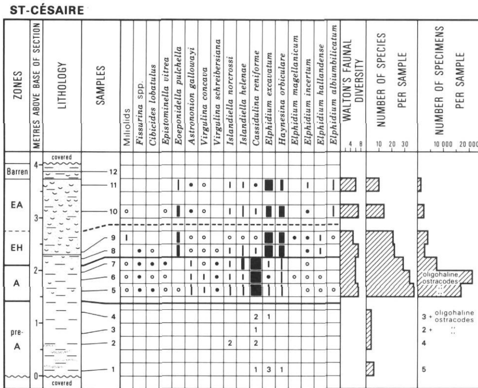
FIGURE 8. Distribution chart for the St-Césaire section. This section is also discussed in LaSalle et al. (1982, p. 16-17 and Fig. 12).
