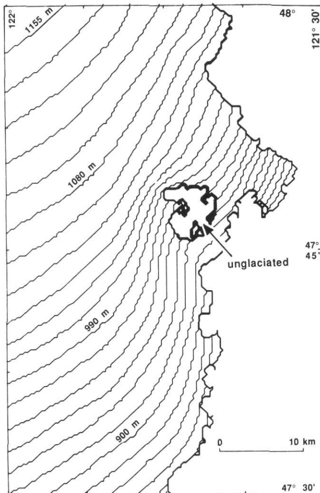
FIGURE 8. Ice-sheet topography of the Puget lobe at maximum stage in the Skykomish-Snoqualmie region (Fig. 6). Contour interval is 15 m.
