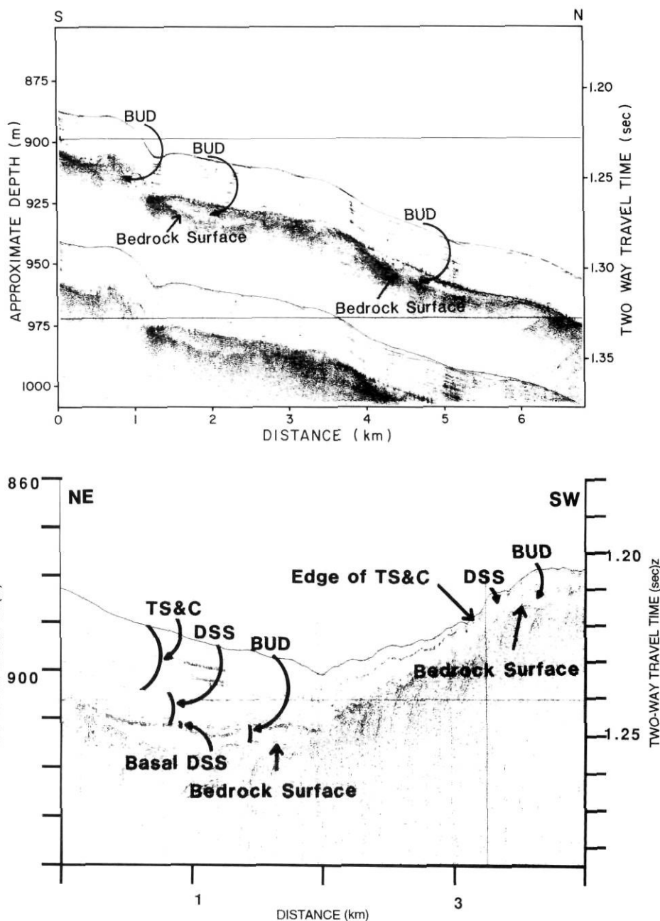
FIGURE 4. A) Huntet profile illustrating the Basal Unstratified Diamict (BUD) infilling bedrock hollows and forming a mound or ridge on bedrock. B) Huntet profile illustrating characteristics of the acoustic units and their vertical relationships. The profile locations are shown in Figure 1. TS&C is the Tiniktartuq Silt & Clay, and DDS is the Davis Strait Silt.
