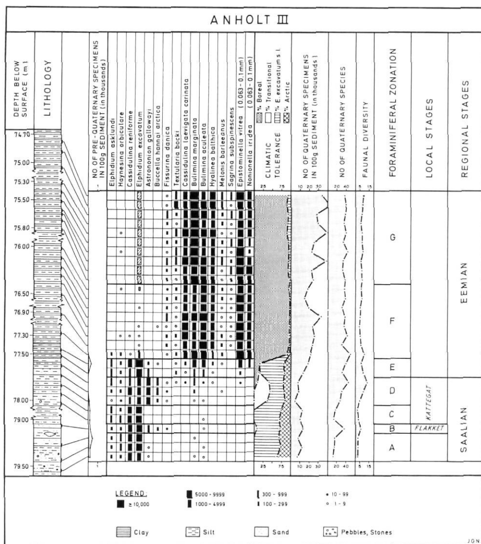
FIGURE 3. Anholt III boring: foraminiferal zones, faunal parameters and concentrations per 100 g sediment of selected benthic foraminifera. Elphidium excavatum s.l.: hatched signature represents dominance of forma selseyensis ; filled in signature represents dominance of forma clavata . Pre-Quaternary foraminifera are mainly re-worked from the Maastrichtian (after Seidenkrantz, 1993a).
