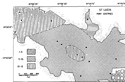
Figure 4 Population density of living Foraminifera in Port Castries, expressed in terms of number of tests per c.c. of wet sediment in the top one-cm layer.
