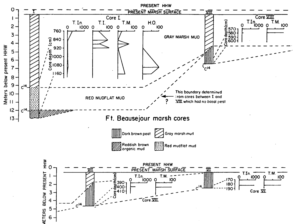
Fig. 13 - Lithologies and foraminiferal occurrences in Ft. Beausejour drill holes. Legend same as Figure 4.
