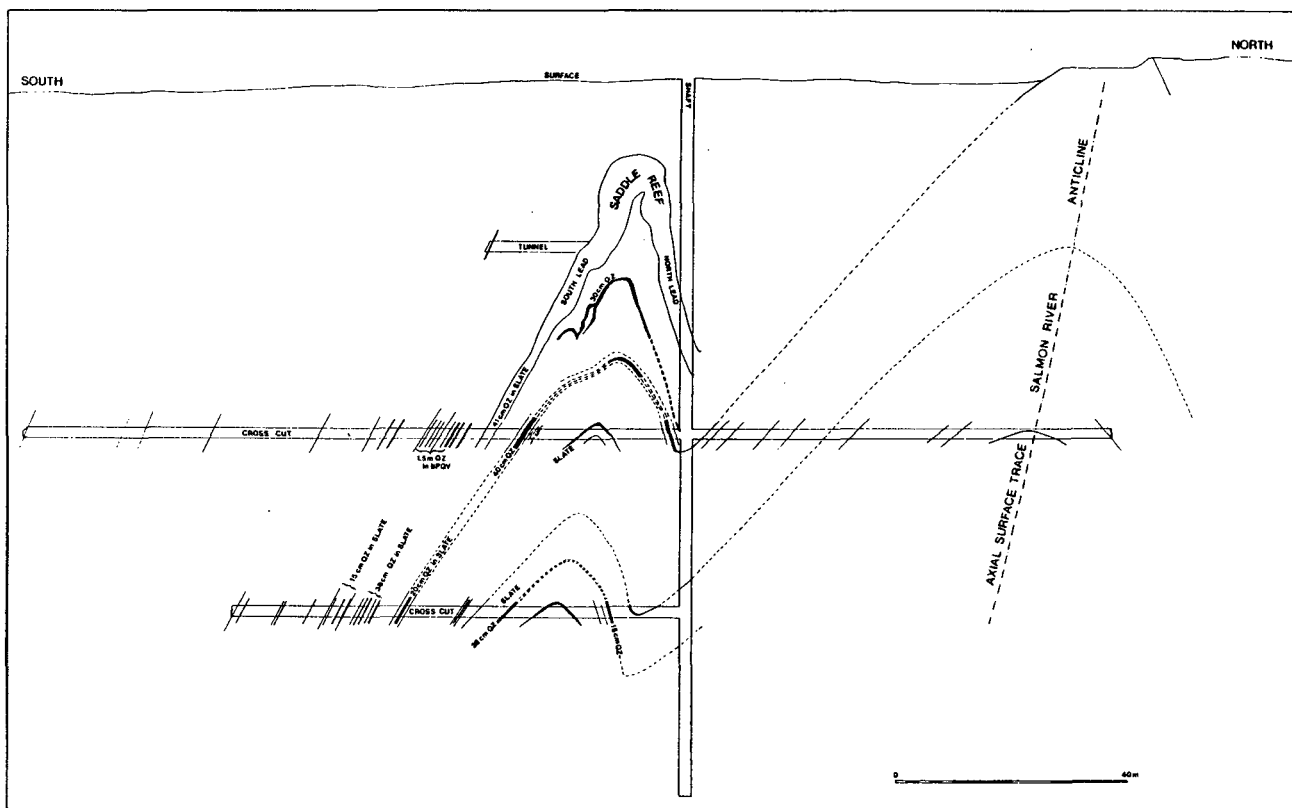
Figure 4 - Transverse-section of the Dufferin Mine, Salmon River Gold District (traced from an unpublished original drawing by E.R. Faribault, Geological Survey of Canada, 1899).
