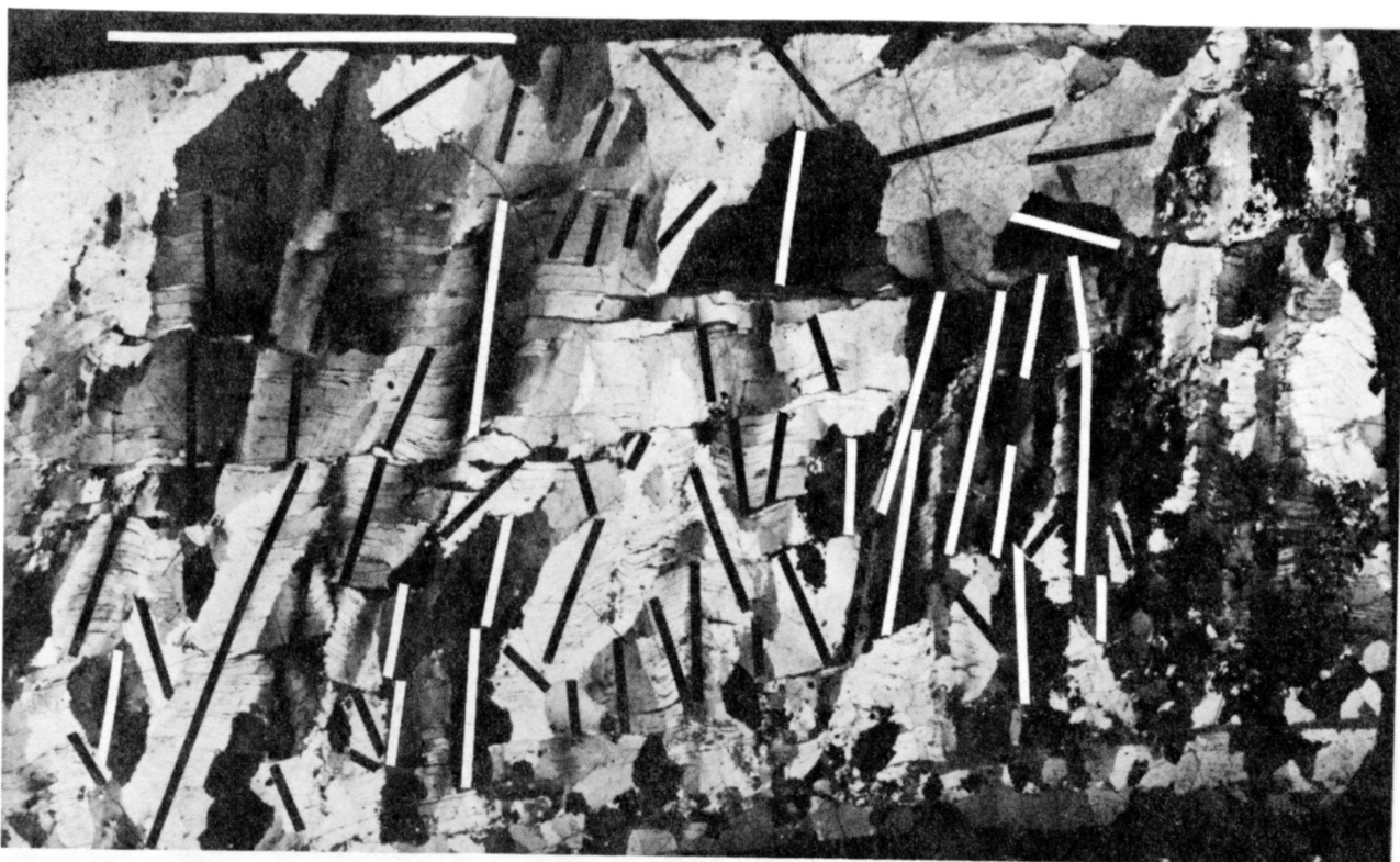
Figure 9 - Photomicrograph of a thin section (cross nicols) of a BP vein at Harrigan Cove Mine (Fig. 6) cut normal to the vein walls, showing the traces of c-axes of quartz crystals (white and black bars). Note the tendency for the c-axes as well as the crystal boundaries to be perpendicular to the laminae which are outlined by trails of white mica, chlorite and opaque material (inclusion bands). The bar scale is 1 cm long. GSC 202510-P
