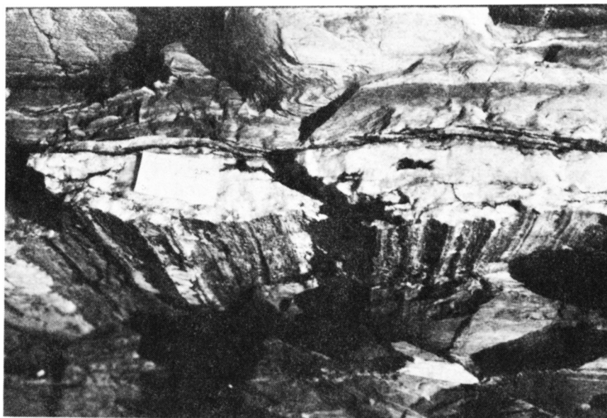
Figure 8 - Photograph of a vertical BP vein showing down-dip grooves on stylolitic laminae. The outcrop is located on the west coast of Liscomb Island, 2 km east of Liscomb Peninsula (LP on Fig. 2). GSC 204124-A
