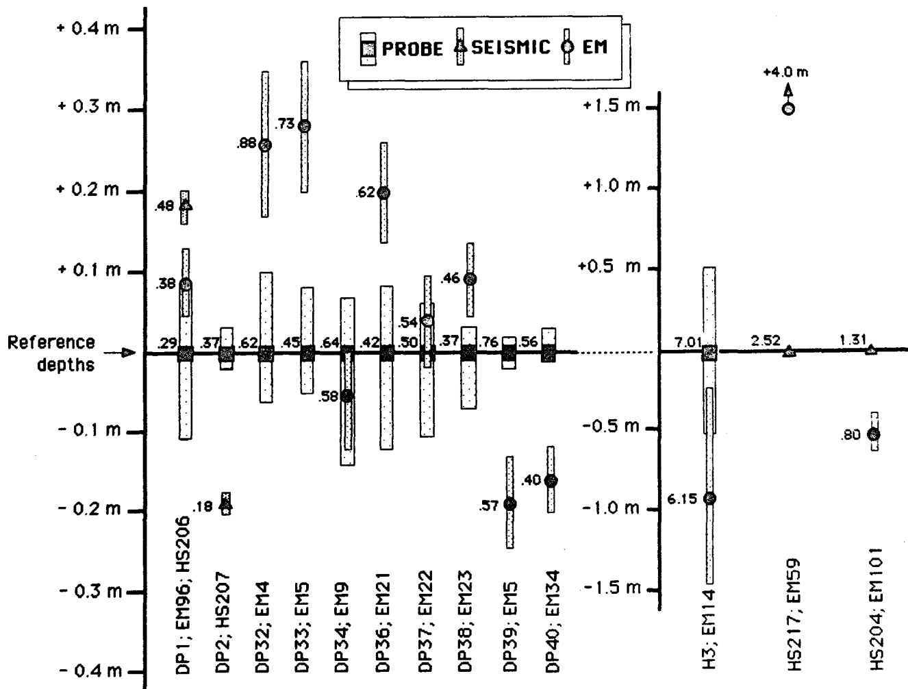
Fig. 4. Comparative results of depth to bedrock for ground truth and geophysical methods (see text for discussion).
