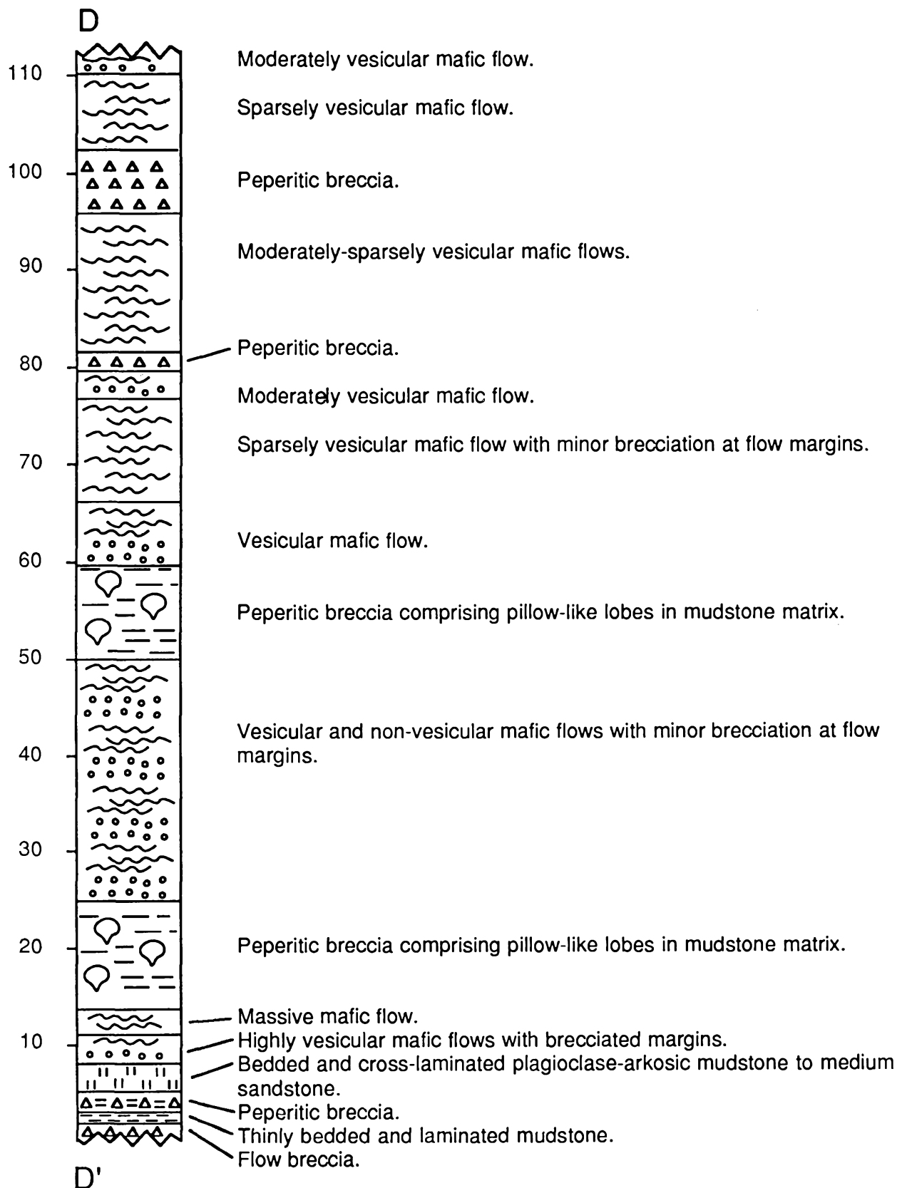
Fig. 4. Representative section of unit Demf2. See Figure 3a for location of section. Scale is in meters.
