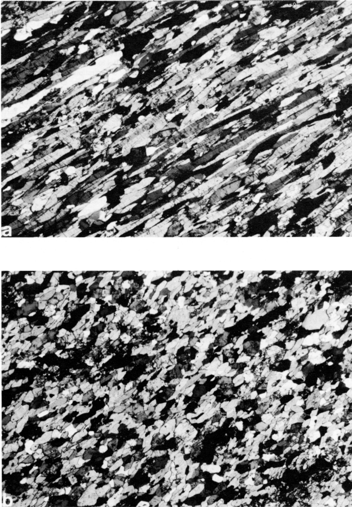
Fig. 3. Photomicrographs of various samples showing classic mylonitic textures. (a) Psammitic or pelitic schist (sample SB-84-153) showing S- and C-surfaces, with mica "fish" and quartz ribbon grains in a groundmass of neoblastic quartz. (b) Mylonitized leucotonalite (sample RR-84-106) showing altered (sericitized) feldspar porphyroclasts in a foliated groundmass of recrystallized quartz and minor chlorite.
