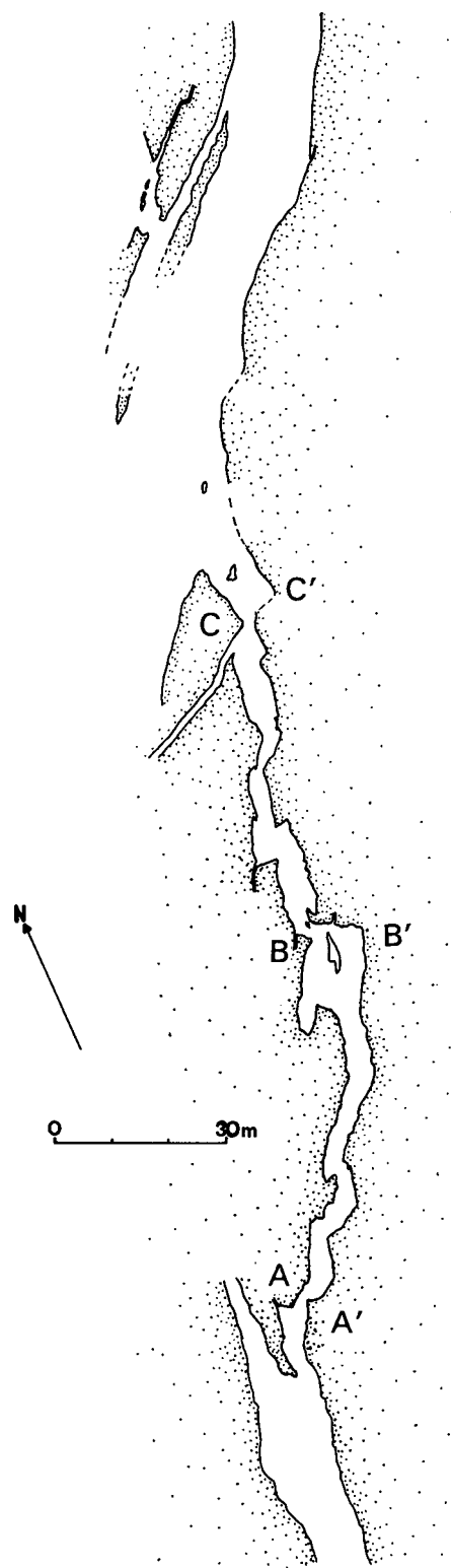
Fig. 5. Map of extensional dykes south of Squally Point, showing the east-west extension recognised from offset of features on conjugate margins. A-A', B-B' and C-C' are examples of conjugate features. Lack of perfect conjugacy is a result of some vertical motion during offset (cf. Fig. 6).
