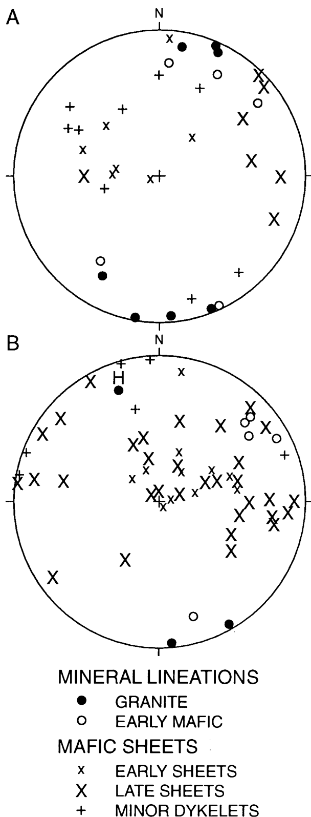
Fig. 7. Stereograms showing orientation of mafic sheets and mineral lineations in (A) West Moose River pluton and (B) North River pluton. H = granite dyke in Harrington River.
