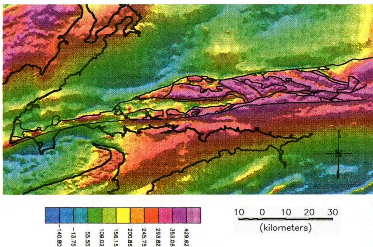
Fig. 9. Magnetic total field map of the Cobequid Highlands. Key to geologic units in Figure 2.
