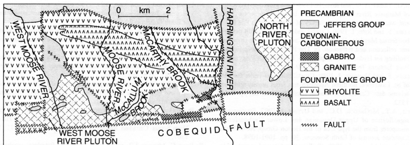
Fig. 11. Map showing distribution of mafic and felsic phases near the West Moose River pluton (modified from Pe-Piper and Turner, 1988a). For explanation, see text.
