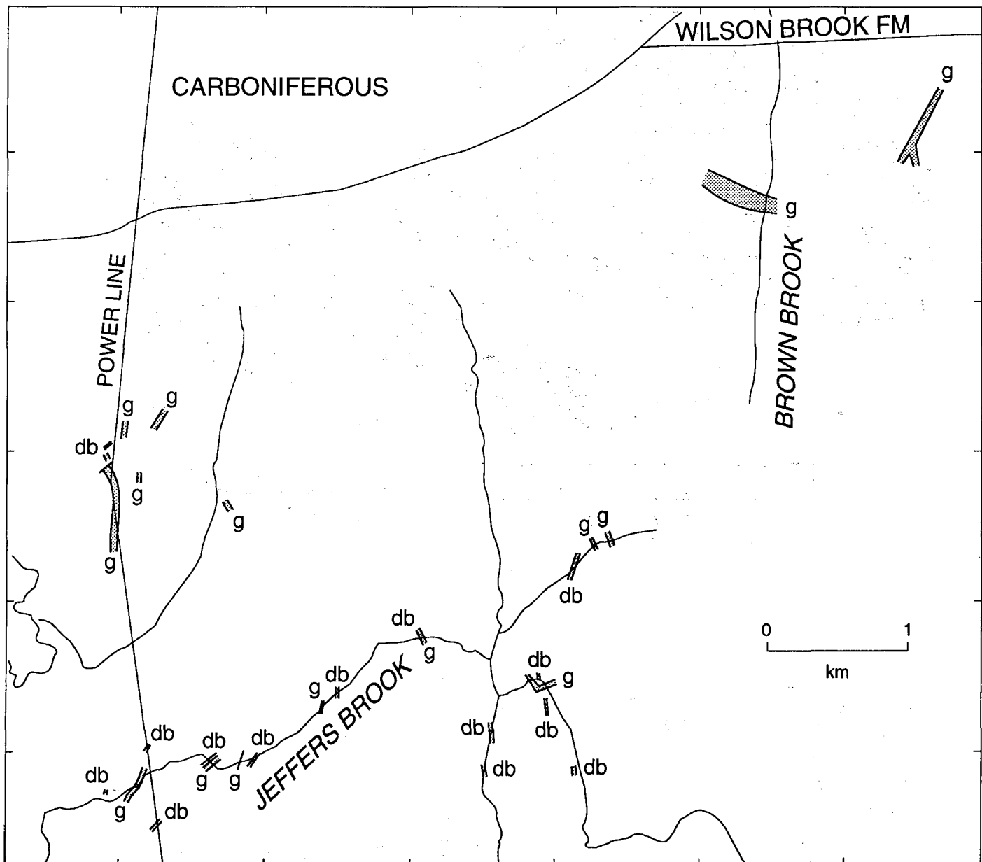
Fig. 8. Map of the area between Jeffers Brook and Brown Brook showing major Carboniferous microgranite and diabase dykes intruded into Neoproterozoic rocks (modified from Pe-Piper and Turner, 1988a). In general, all brook and powerline sections have been examined for dykes.
