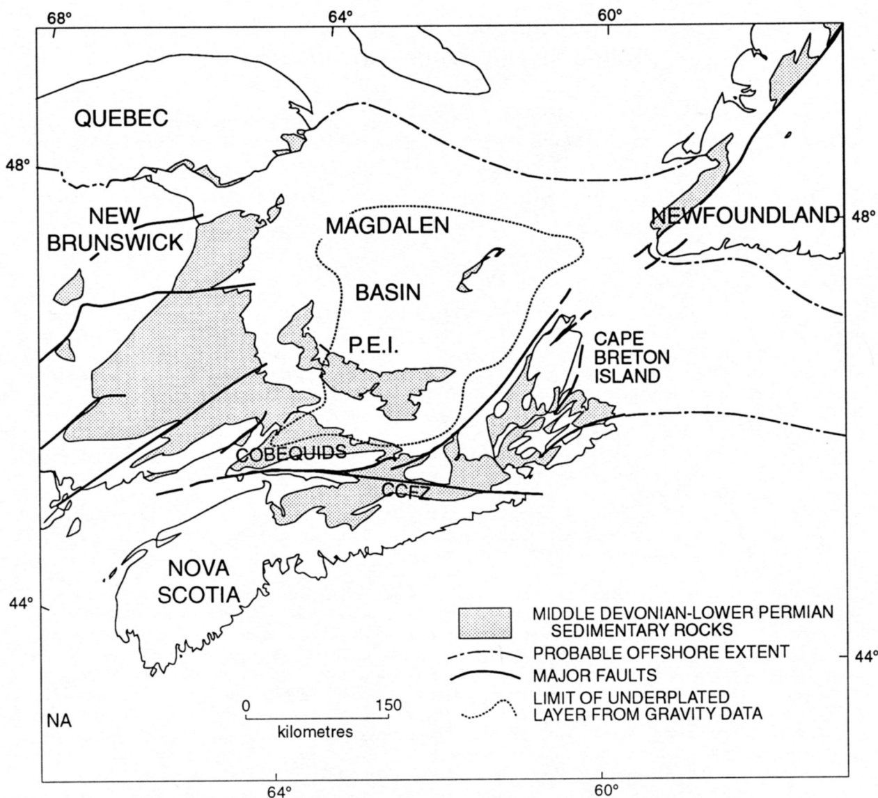
Fig. 1. Regional map showing tectonic setting of the Cobequid Highlands within the larger Magdalen Basin (stippled area). CCFZ = Cobequid-Chedabucto Fault zone.
