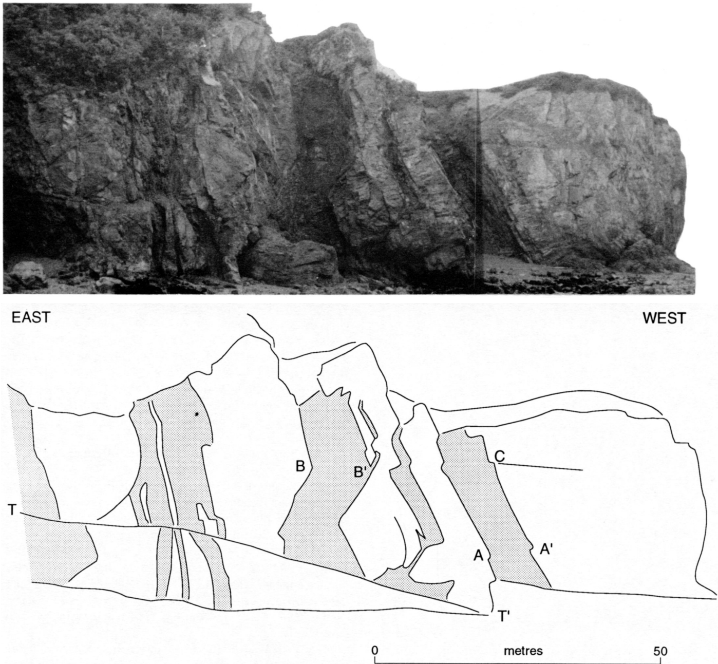
Fig. 6. Photograph and annotated sketch of late dykes cutting Fountain Lake Group rhyolites immediately east of Squally Point. T-T' is thrust plane. A-A', B-B' are examples of conjugate dyke margins. C is minor offset of dyke along flat-lying plane.
