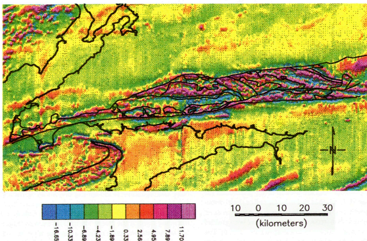
Fig. 10. Magnetic first vertical derivative map of the Cobequid Highlands. Key to geologic units in Figure 2.
