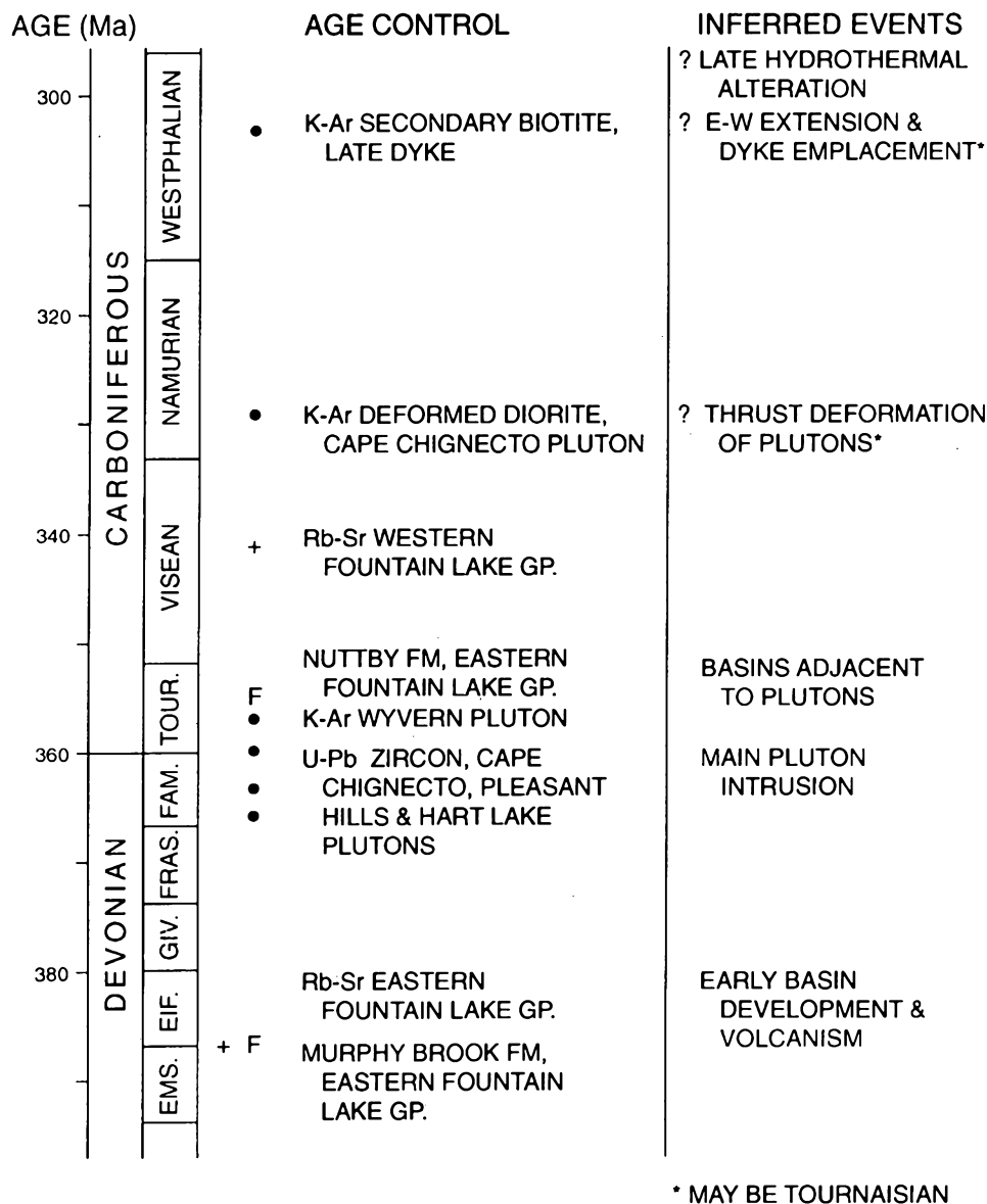
Fig. 3. Stratigraphic column showing available chronology and key Devonian-Carboniferous events in the Cobequid Highlands (modified from Nearing, 1992). F = fossil determinations from Donohoe and Wallace (1982, 1985). • = K/Ar and U/Pb radiometric age determinations for intrusive rocks (from Pe-Piper and Piper, 1987; Waldron et al. , 1989; Doig et al. , 1991). + = Rb/Sr "isochrons" for volcanic rocks from Pe-Piper et al. (1989). Errors on U-Pb ages are about \pm 3 Ma, on K/Ar ages about \pm 10 Ma, and on Rb/Sr ages on volcanic rocks \pm 4 Ma. Note that interpretation of younger events is based only on K/Ar dates: these events may be older (cf. Pe-Piper and Koukouvelas, in press).
