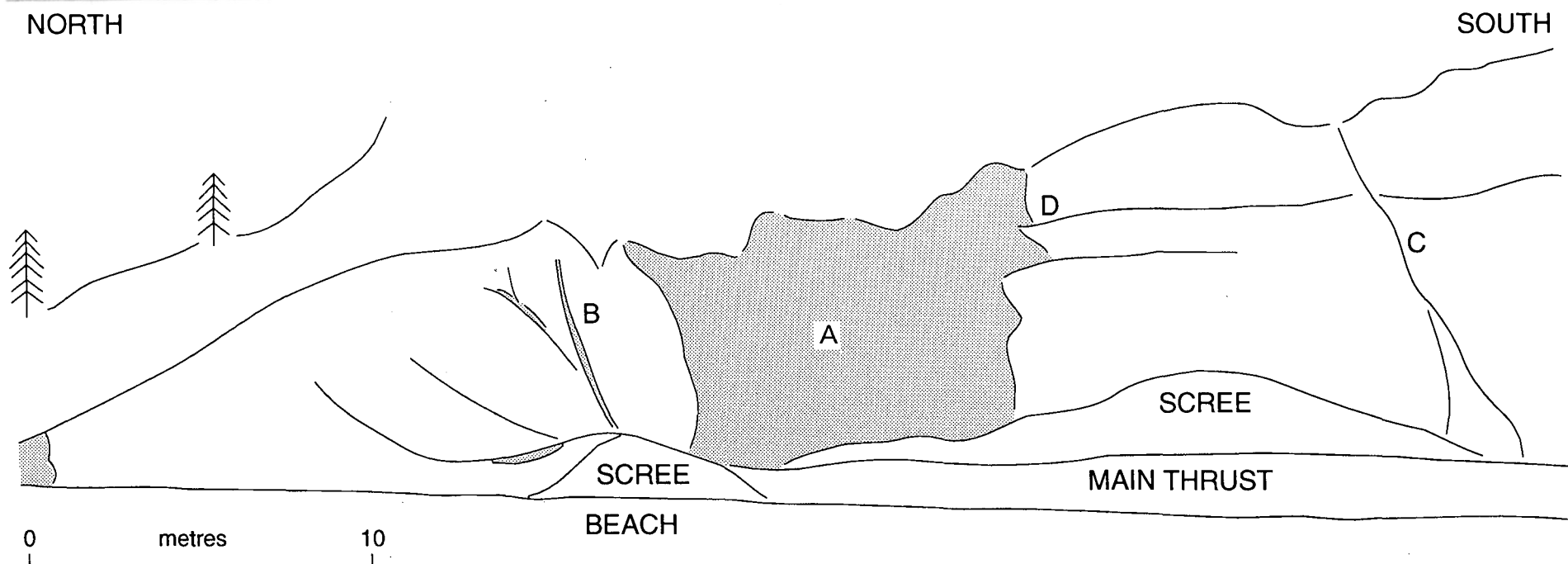
Fig. 4. Photograph and annotated sketch of thrust and ramp features in Fountain Lake Group rhyolites south of Squally Point. (A) early dyke striking 040^{\circ} cut by main thrust; (B) minor diabase bodies, relatively undeformed, occupying splays of main thrust; (C) diabase dyke with 040^{\circ} shear zone contact with rhyolite; (D) minor offsets of dyke on flat-lying planes.
