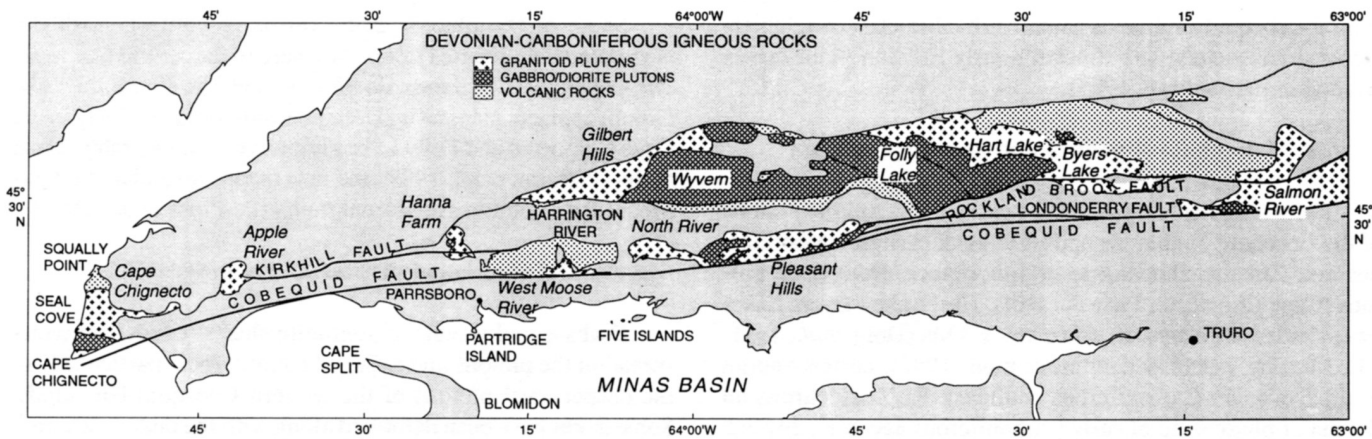
Fig. 2. Summary geological map of the Cobequid Highlands showing distribution of Devonian-Carboniferous igneous rocks. Boundaries modified from Donohoe and Wallace (1982) on the basis of our mapping and magnetic data.
