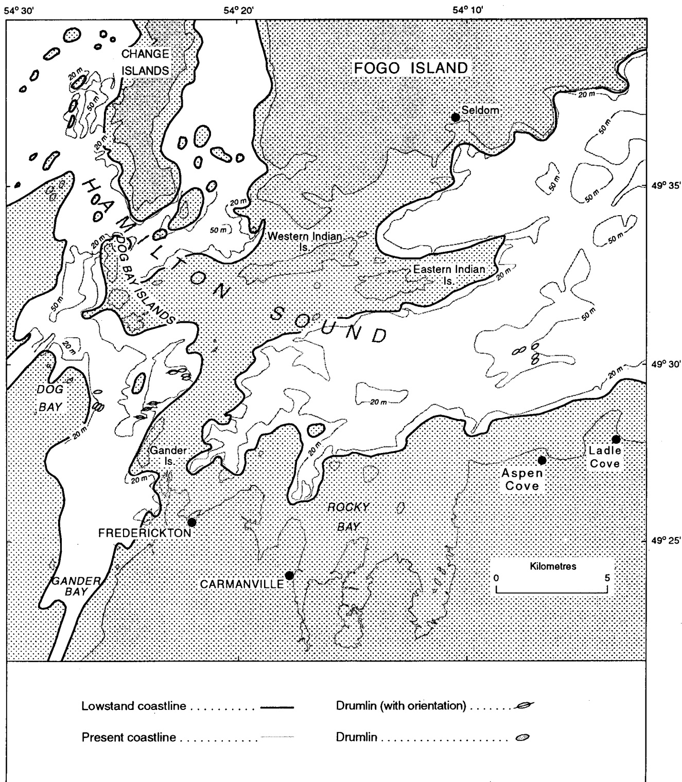
Fig. 10. The present coastline of the study area and the coastline during the early Holocene postglacial relative sea-level minimum. Also shown are the positions of drumlins (which were not emergent).
