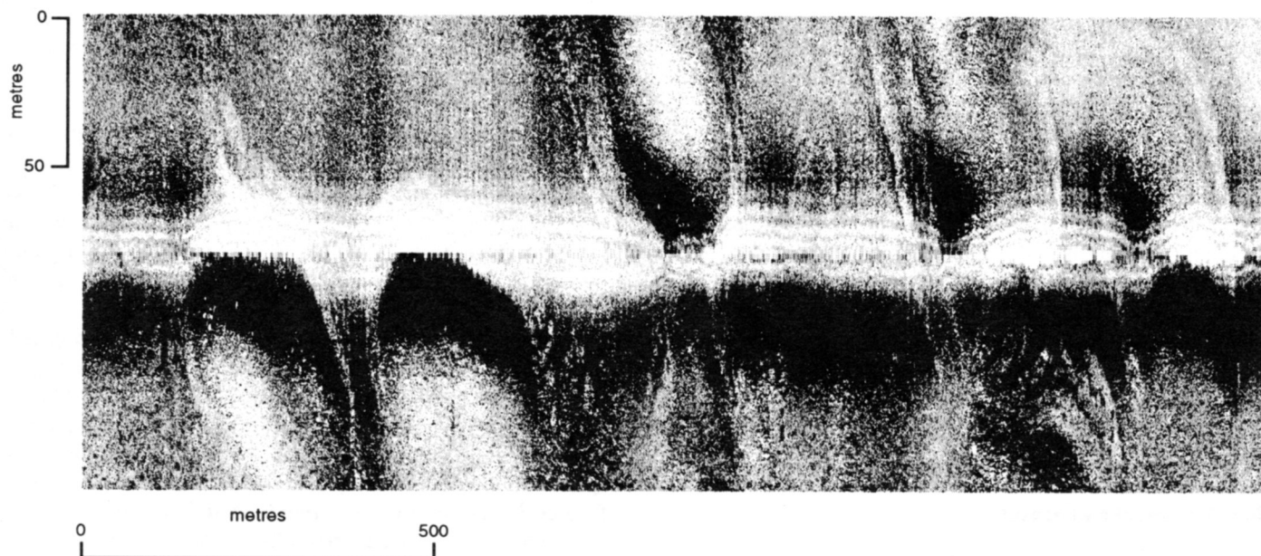
Fig. 4. Sidescan sonar image of a series of small drumlins northwest of Gander Island (location shown on Fig. 2). The orientation of the drumlins is 160 degrees.
