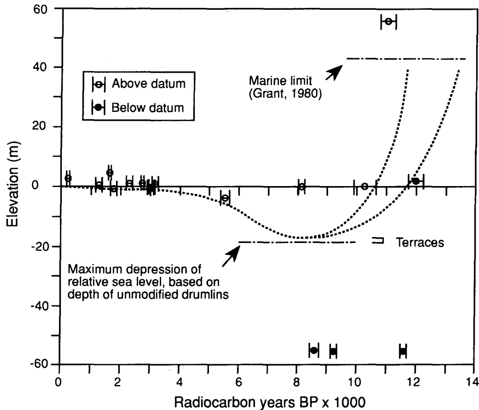
Fig. 9. Relative sea-level curve for the Hamilton Sound region. Data on index points are shown on Table 1. The marine limit is from Grant (1980); Catto (1993) reported a higher limit. The depth of the lowstand is constrained by unmodified drumlin crests at -19 m and wave-cut terraces at depths between 17 and 21 m. We are reasonably confident of the accuracy of the portion of the curve postdating 8 ka B.P., but less so of the older part. Consequently, the pre- 8 ka B.P. portion is represented by an envelope contained within the two lines.
