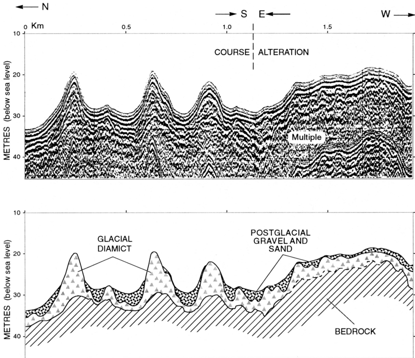
Fig. 6. Seistec high-resolution seismic reflection profile across drumlins at the mouth of Gander Bay (Fig. 2). The drumlins extend 15 m above the surrounding seabed.
