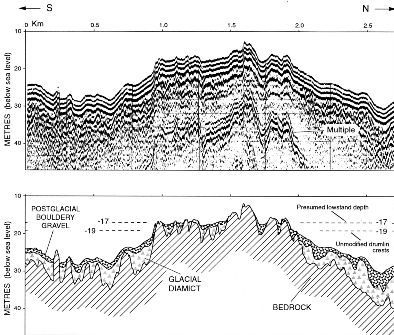
Fig. 8. Seistec high-resolution seismic reflection profile across a terrace north of Fredericton (location shown on Fig. 2). Depth of the terrace surface ranges from 15 m to 18 m below MSL. The surface is bouldery gravel with scattered bedrock outcrops. Below a depth of 18 m gravel completely masks bedrock or glacial diamict. Because of the intense ringing (across ~6 m) on Bubble Pulser records it is difficult to resolve the stratigraphy in detail.
