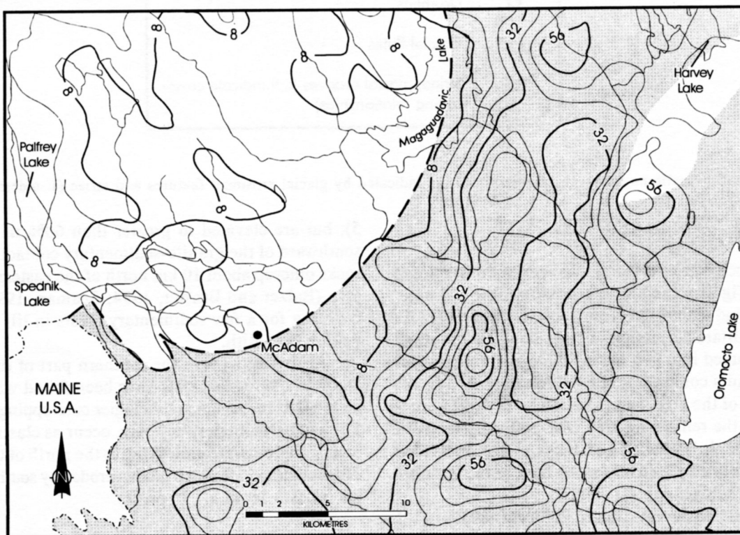
Fig. 5. Percent sedimentary rock clasts till. The shaded area denotes Silurian to Pennsylvanian sedimentary bedrock in the McAdam area.
