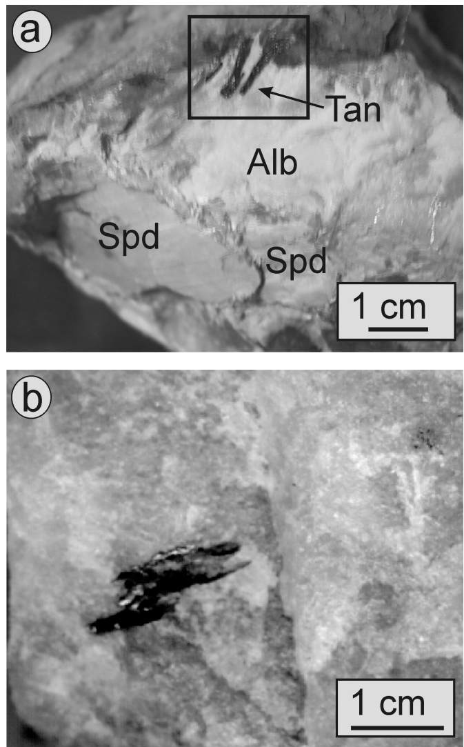
Fig. 3 (a) Sample of coarse-grained, intergranular spodumene (Spd)-albite (Alb)-muscovite (at the contact of Spd-Alb) material with euhedral blades of tantalite (Tan; within the box area). (b) Photograph of molybdenite flake (sample BRZ-2002-1 of Table 2) of ca. 1 cm size in quartzite from adjacent to Brazil Lake pegmatite. Finer grained molybdenite grains (sample BRZ-2002-2 of Table 2) were liberated from this sample upon crushing. Note the purity of the sample is (i.e., silica-rich) and its fine-grained, saccharoidal texture.
