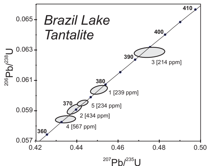
Fig. 4 Conventional concordia plot displaying U-Pb analyses for tantalite grains from Brazil Lake pegmatite (Fig. 3a).
