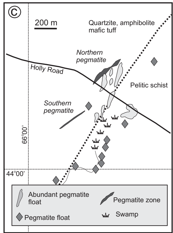
Fig. 1 (a) Regional setting and geology of the Meguma terrane in the Appalachian Orogen. (b) Regional geological map of southwestern Nova Scotia (modified after White et al. 2001) showing the location of the Brazil Lake pegmatite (BLP), location of the former producing East Kemptville tin - base metal deposit, and extent of regional shear zones in this area (TSZ – Tobeatic Shear Zone, EKSZ – East Kemptville Shear Zone, CP-DSZ – Chebogue Point-Deerfield Shear Zone, CPSZ – Cranberry Point Shear Zone). (c) Map outlining extent of the Brazil Lake pegmatite field. Note that the extent of the northern pegmatite lens is based on diamond drill holes. The samples used in this study come from the southern pegmatite outcrop. Figure modified after map provided by D. Black (personal communication 2004).
