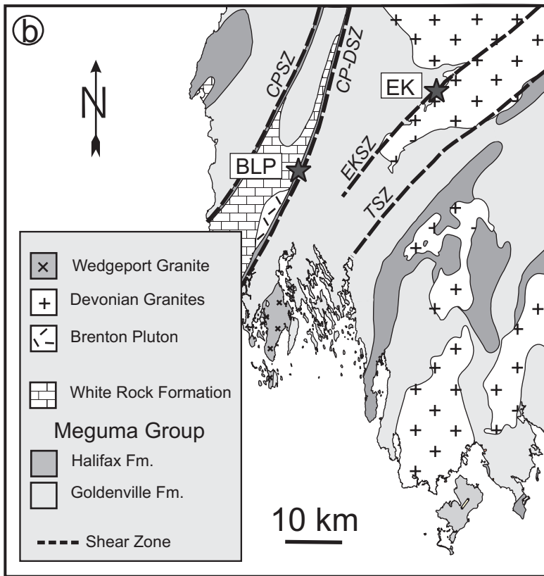
Fig. 1 (a) Regional setting and geology of the Meguma terrane in the Appalachian Orogen. (b) Regional geological map of southwestern Nova Scotia (modified after White et al. 2001) showing the location of the Brazil Lake pegmatite (BLP), location of the former producing East Kemptville tin - base metal deposit, and extent of regional shear zones in this area (TSZ – Tobeatic Shear Zone, EKSZ – East Kemptville Shear Zone, CP-DSZ – Chebogue Point-Deerfield Shear Zone, CPSZ – Cranberry Point Shear Zone). (c) Map outlining extent of the Brazil Lake pegmatite field. Note that the extent of the northern pegmatite lens is based on diamond drill holes. The samples used in this study come from the southern pegmatite outcrop. Figure modified after map provided by D. Black (personal communication 2004).
