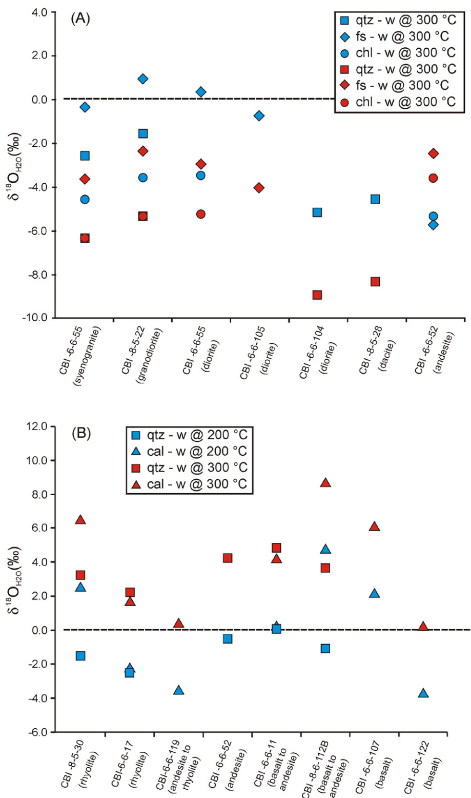
Fig. 6. Hydrothermal fluid compositions ( \delta^{18}\text{O}_{\text{H}_2\text{O}} ) for: (A) propylitic assemblage minerals at 300 and 450 °C, and (B) quartz-sericite-calcite assemblage minerals at 200 and 300 °C. The mineral- \text{H}_2\text{O} oxygen-isotope geothermometers utilized are: calcite- \text{H}_2\text{O} (Friedman and O'Neil 1977), chlorite- \text{H}_2\text{O} (Wenner and Taylor 1971), alkali feldspar- \text{H}_2\text{O} (O'Neil and Taylor 1967) and quartz- \text{H}_2\text{O} (Matsuhisa et al. 1979). Abbreviations: cal - calcite, chl - chlorite, fs - feldspar, qtz - quartz.
