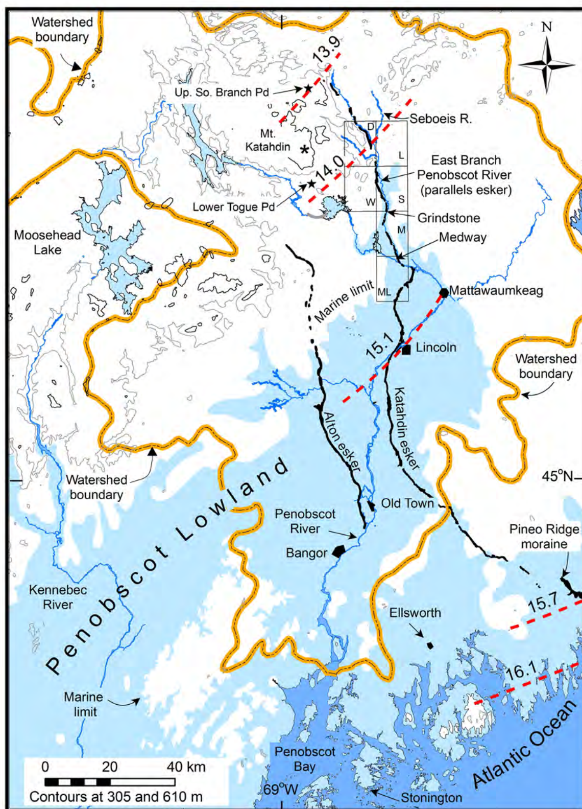
Figure 1. Map of part of Maine showing the Penobscot River, its drainage basin, and locations mentioned in the text. Light blue areas on land were submerged during the high stand of sea level at ~14 ka. Light grey contours are at 305 m and darker ones are at 610 m asl. Marine limit and Pineo Ridge moraine from Thompson and Borns (1985a). Red dashed lines are approximate ice-margin retreat isochrones. The 7½ minute quadrangles used in the study are outlined. D = Deasey Mtn., L= Lookout Mtn., W= Whetstone Mtn., S=Stacyville, M=Millinocket East, and ML= Medunkeunk Lake.
