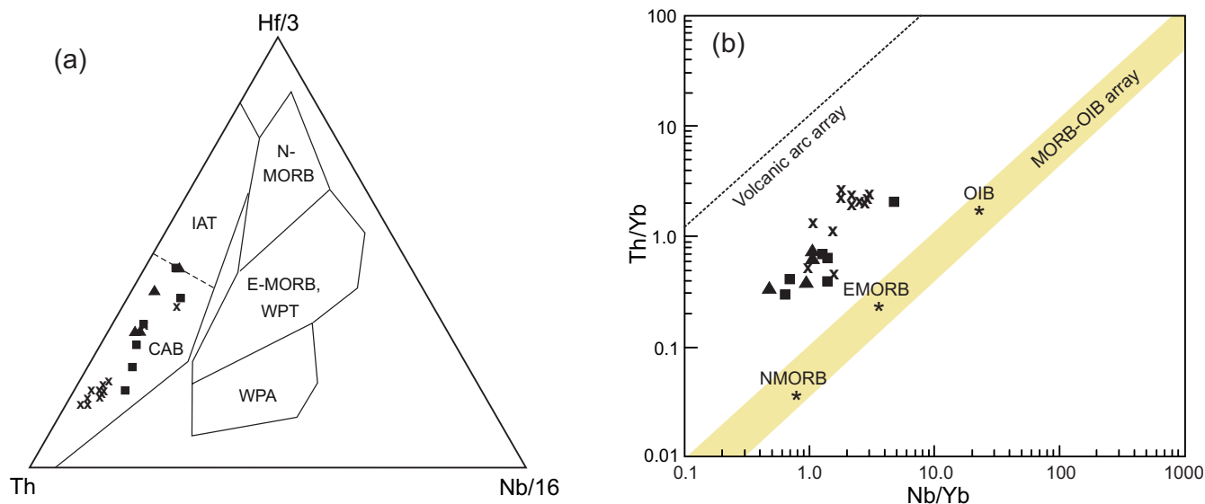
Figure 12. Tectonic discrimination diagrams comparing the Almond Road and Belleisle Bay groups: (a) ternary Th-Hf-Nb diagram with fields defined by Wood (1980) and (b) bivariate Th/Yb vs Nb/Yb diagram after Pearce (2008). Abbreviations: CAB – calc-alkaline basalt; E-MORB – enriched mid-ocean ridge basalt; N-MORB – normal mid-ocean ridge basalt; IAT – island arc tholeiite; WPA – within-plate alkalic basalt; WPT – within-plate tholeiitic basalt. Symbols same as in Figure 10.
