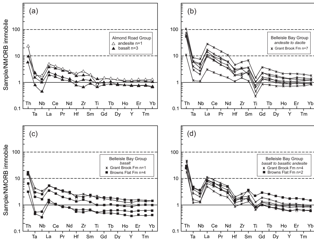
Figure 11. N-MORB-normalized spider diagrams after Sun and McDonough (1989) in Pearce (2014) showing mafic to intermediate volcanic rocks of the Almond Road and Belleisle Bay groups: (a) Almond Road Group andesite and basalt; (b) Grant Brook Formation andesite to dacite; and (c, d) Grant Brook and Browns Flat formations basalt to basaltic andesite.
