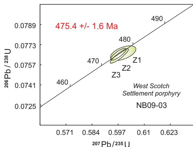
Figure 7. Concordia diagram for NB09-03. Analytical data listed in Table 1.
