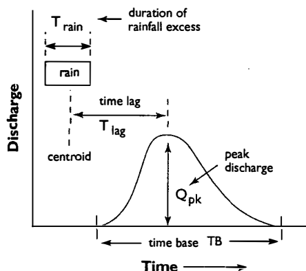
FIGURE 2 UNIT HYDROGRAPH
