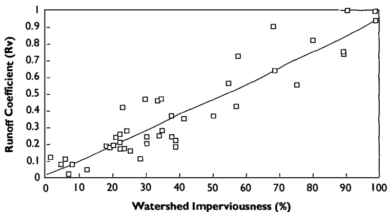
FIGURE 1 IMPERVIOUSNESS AND STORMWATER RUNOFF IN A WATERSHED
