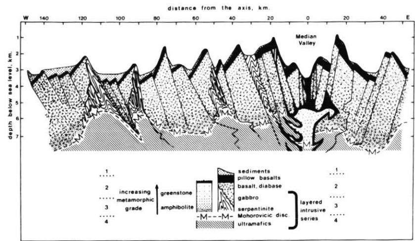
Schematic cross-section through the oceanic crust beneath the Mid-Atlantic Ridge at 45°N.
