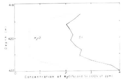
Figure 8 Change in chemistry across one lava flow from Bermuda. Potassium as K_2O (%) and strontium (100's of ppm) against depth in the bore-hole. (From Aumento and Gunn, 1975).
