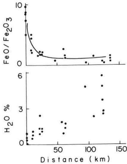
Figure 6 Changes in weathering with distance from a ridge axis. Oxidation ratio FeO/Fe_2O_3 (upper), and % water (lower), versus distance from the axis of the Mid-Atlantic Ridge at 45°N (from Irving, 1970).
