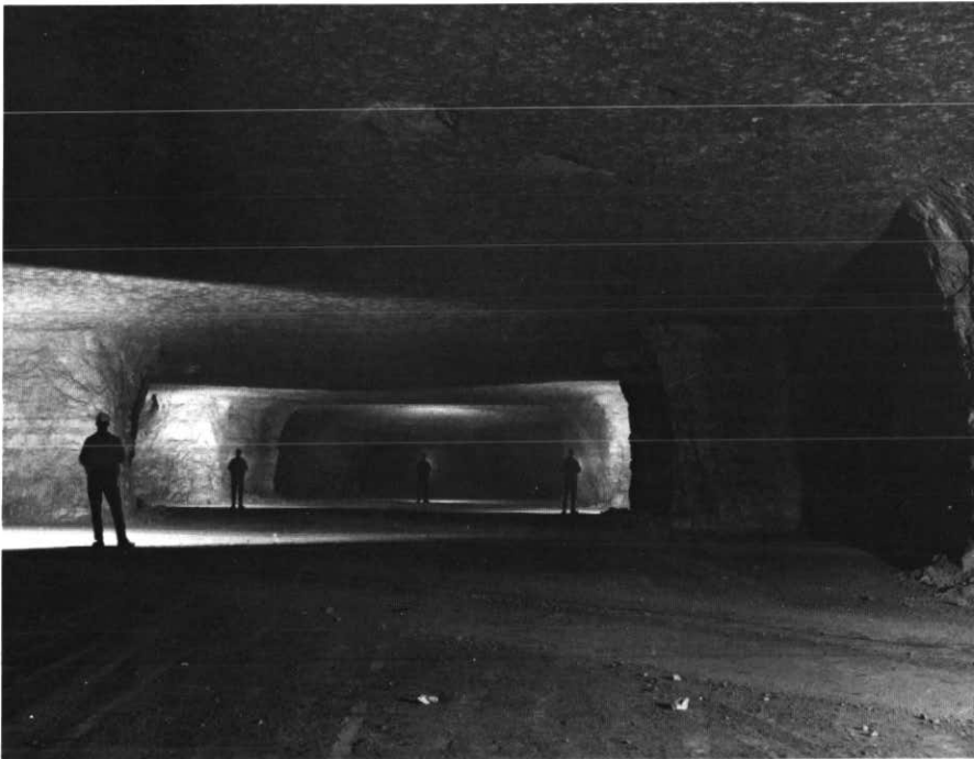
Figure 2. View inside one of the disused mined-out areas at Kansas City in the Bethany Falls limestone. This shows a level floor and competent rock roof; developments noted in
