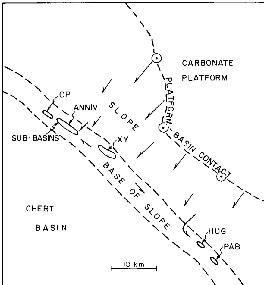
Figure 12 General model for the formation of the platform-marginal deposits showing the geometry of the platform-slope-base of slope and chert basin facies. Arrows show surface
