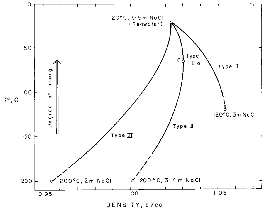
Figure 15 The evolution of brines (NaCl solutions) as they mix with seawater, showing temperature and density. Note Type II changes at point C forming brine Type IIa, (after Sato, 1972).
