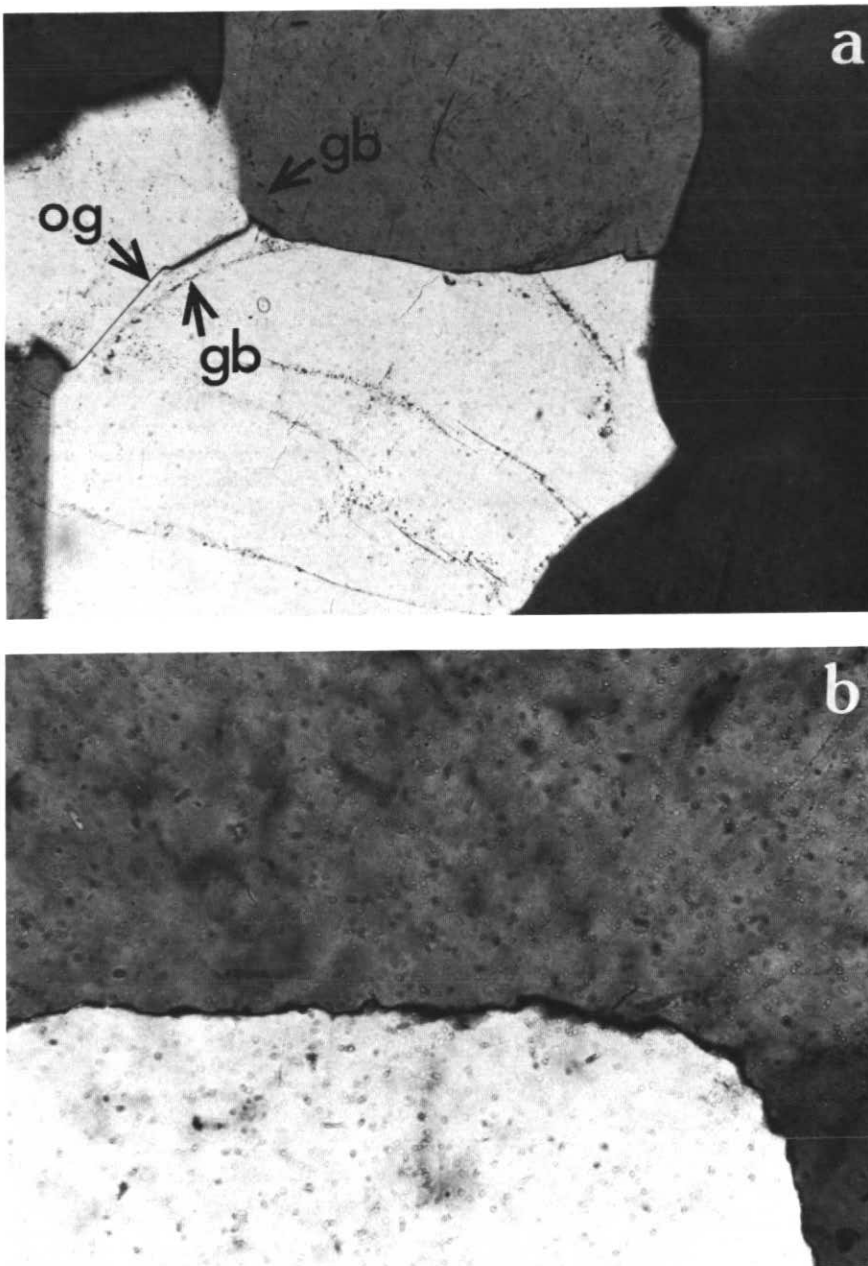
Figure 3 These photomicrographs show textures commonly associated with pressure solution. In 3a (60 X) quartz grains show "dust rings" where the original grain boundary (gb) has been overgrown by euhedral quartz (og). The concavo-
