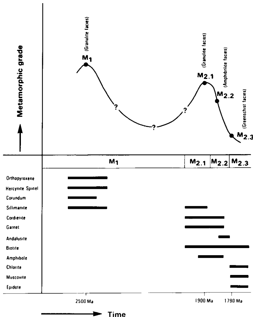
Figure 13 Path of metamorphism and related mineral growth in rocks of the Canadian Shield
