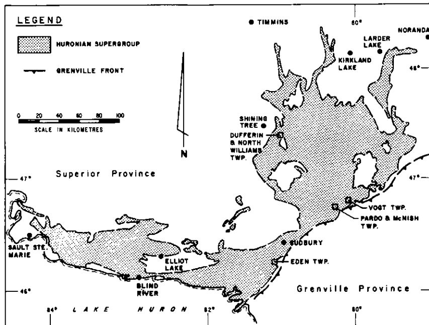
Figure 1 Distribution of Huronian Supergroup (stippled); bulge northeast of Sudbury is the Cobalt Embayment. Note the digitation of
