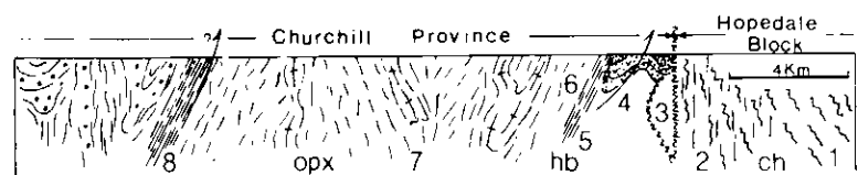
Figure 4 Schematic SE to NW cross-section of the Hopedale block and the eastern Churchill Province (Section C, Figure 2). Isograds: ch, chlorite (and epidote) in cross-cutting schistosity; hb, hornblende (and diopside + garnet); opx, orthopyroxene. Numbers refer to zones described in text.
