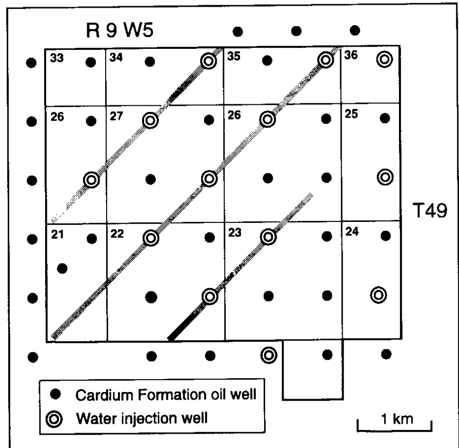
Figure 19 Connections between injection wells drilled to recover oil from the Cretaceous Cardium formation in the Pembina oil field, Alberta (redrawn from McLeod, 1977). Water injected at pressures greater than the overburden load produced hydraulic fractures that propagated to the NE and SW. This is consistent with S_{Hmax} orientations inferred from breakouts in nearby wells.
