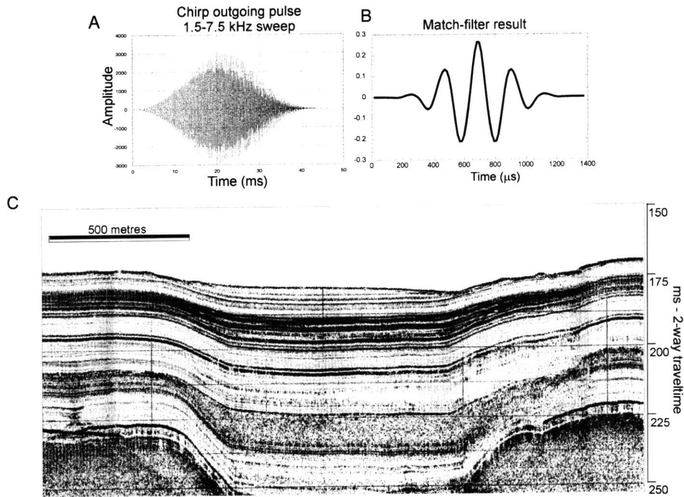
Figure 3 (A) is a chirp sonar 1.5-7.5 kHz swept outgoing pulse and (B) same source function after match-filtering (data compliments of M. Jakobsson). (C) is an example of a chirp profile from Lake Huron collected with a Datasonics CAP 6000 profiler with a 100 ms pulse length swept from 4 - 10 kHz (image courtesy of L. Mayer).
