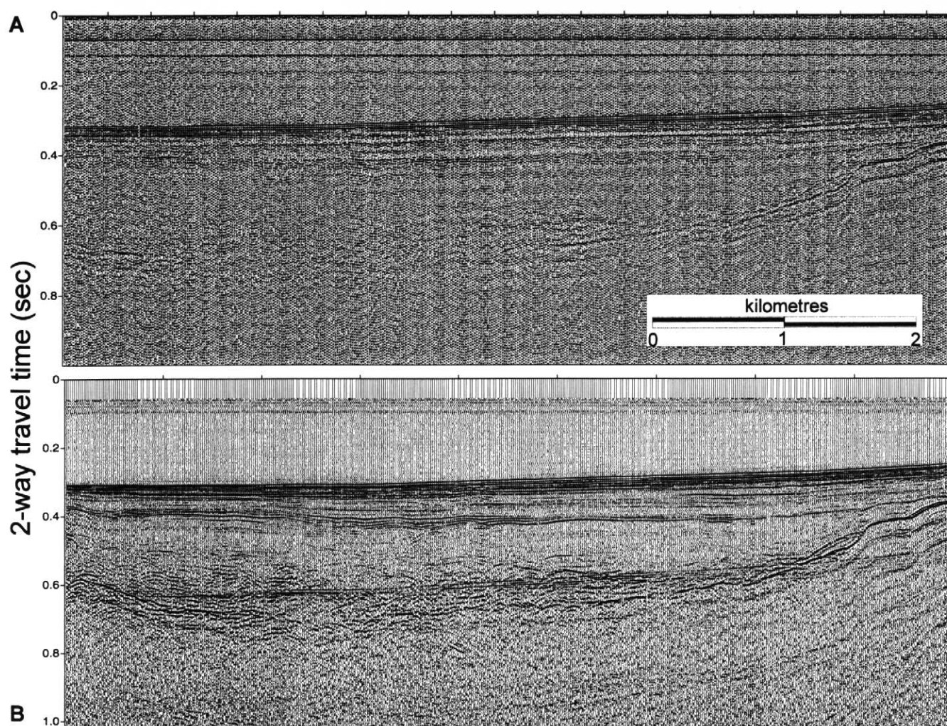
Figure 9 A 10 in 3 airgun profile from Saanich Inlet, BC: (A) is a single channel profile extracted from the multichannel array, and (B) is the 6-fold stacked record from the 24-channel array. There is abundant coherent noise on the single channel record, the result of a faulty digitizing board. The stacked section (B) highlights the improvements that can be achieved in the signal-to-noise ratio through move-out and stacking in multichannel array processing.
