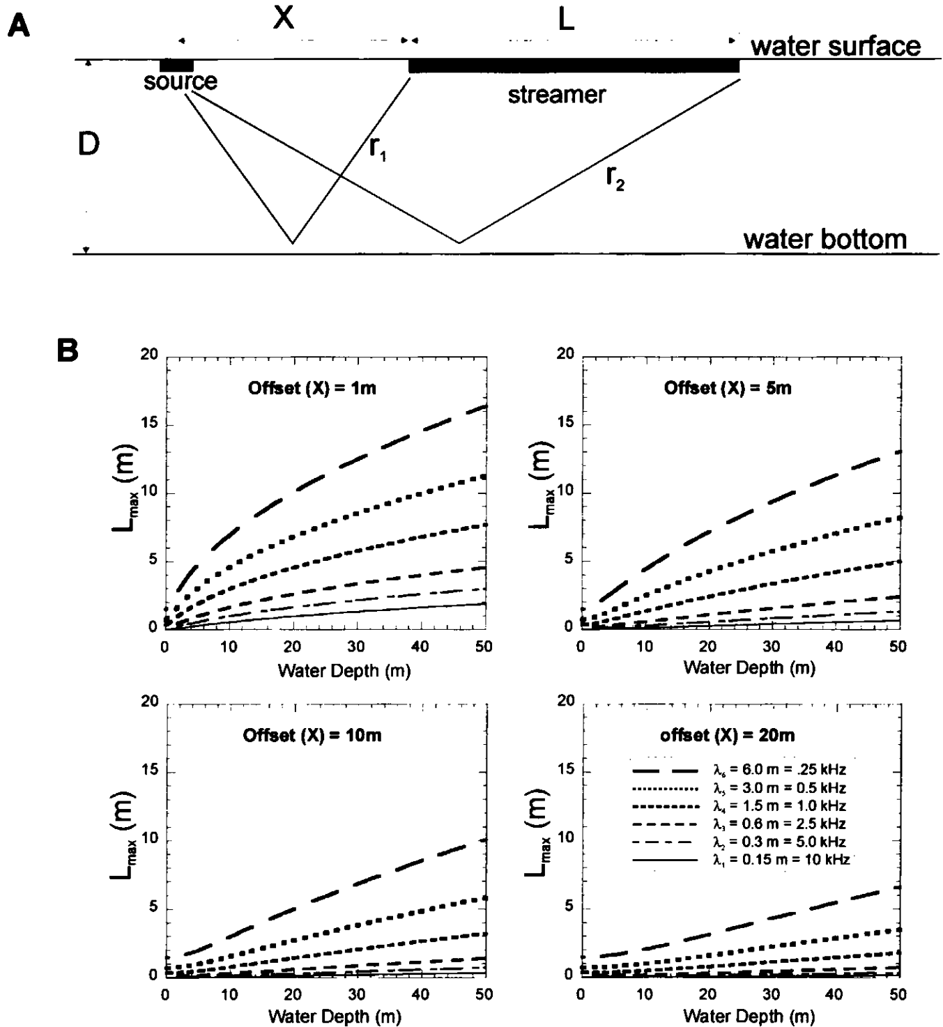
Figure 8 (A) Schematic of commonly used source-receiver geometry. (B) Relationship between water depth (D), source-receiver offset (X), minimum wavelength ( \lambda_1 ) or highest frequency of interest and maximum array length ( L_{\max} ) for source-receiver geometry as shown in A, and described in equation 6. Modified from Verbeek and McGee (1995).
