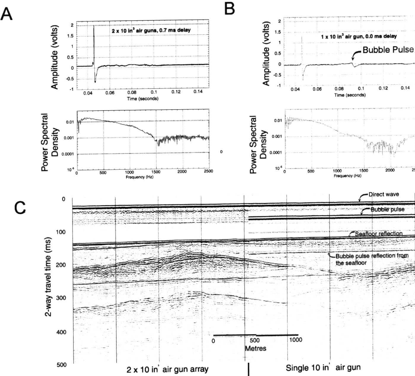
Figure 5 (A) shows a source function for a 2 x 10 3 in 3 tuned airgun array compared with (B), a single 10 3 in 3 airgun source function. (C) is an example profile in the eastern Strait of Juan de Fuca resulting from first, the two gun array shown in A, then the single 10 3 in 3 airgun. Note the lower energy levels (lower gain) in the second part of the profile and the predominance of the bubble pulse.
