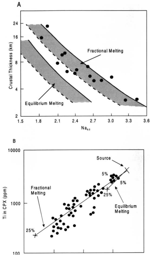
Figure 4 (A) Average Na contents of MORB (normalized to 8 wt% MgO) versus crustal thickness determined seismically, showing modelled results for different melting processes (After Langmuir et al. , 1992). (B) Clinopyroxene (Cpx) compositions from abyssal peridotites compared to trends from different melting processes (Johnson et al. , 1990). These plots suggest that fractional or “near fractional” melting is the dominant process in generating MORB melts.
