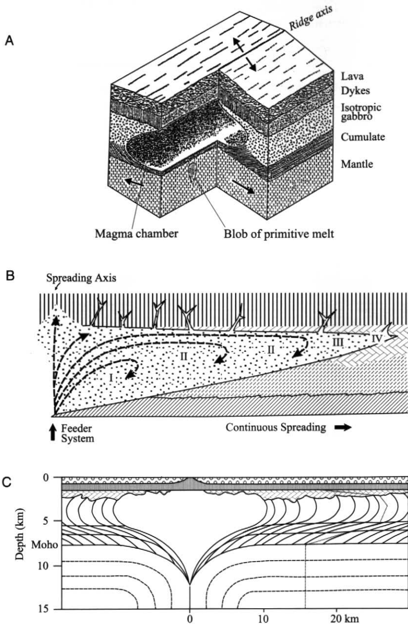
Figure 9 Various concepts of large, single magma chambers derived from ophiolite studies. (A) the "infinite onion" model; (B) the "wing-shaped" model; and (C) the "axial trough model" (references in text).
