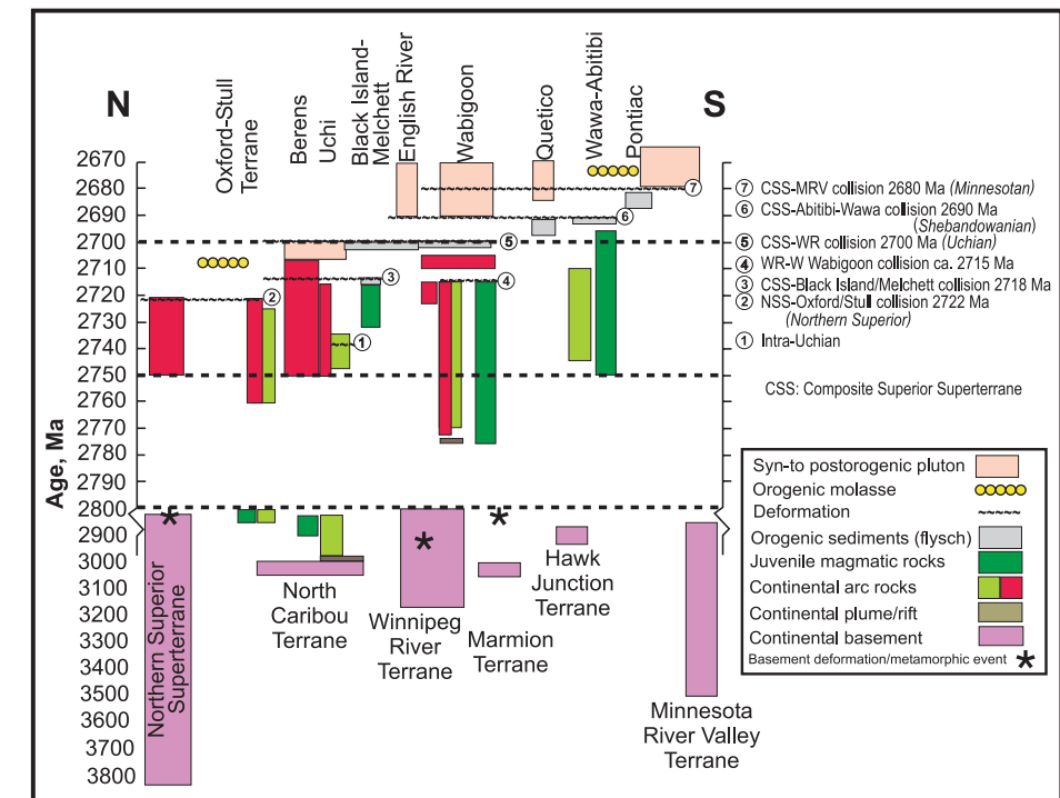
Figure 11 Cladogram (cf. Hoffman, 1989) illustrating timing of assembly of the Superior Province from continental and oceanic fragments. Note successive merging of terranes between 2720 and 2680 Ma.
