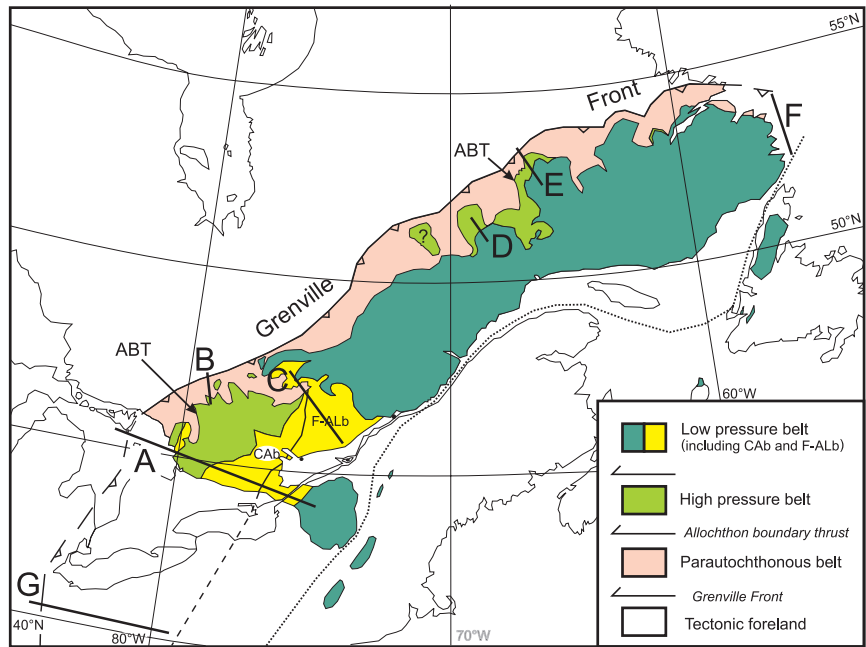
Figure 6 Sketch map of the Grenville Province showing the distribution of orogen-scale belts (after Rivers et al., 2002). Thick lines labeled A to G are the locations of seismic transects. ABT: Allochthon boundary thrust; CAB: Composite Arc belt; F-ALb: Frontenac-Adirondack Lowland belt.
