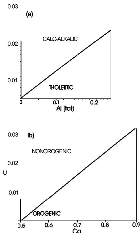
Figure 4. Bivariate diagrams (Letterier et al. 1982) showing how the chemical composition of clinopyroxene reflects the (a) calc-alkalic vs tholeiitic, and (b) orogenic vs non-orogenic conditions in which it formed.
