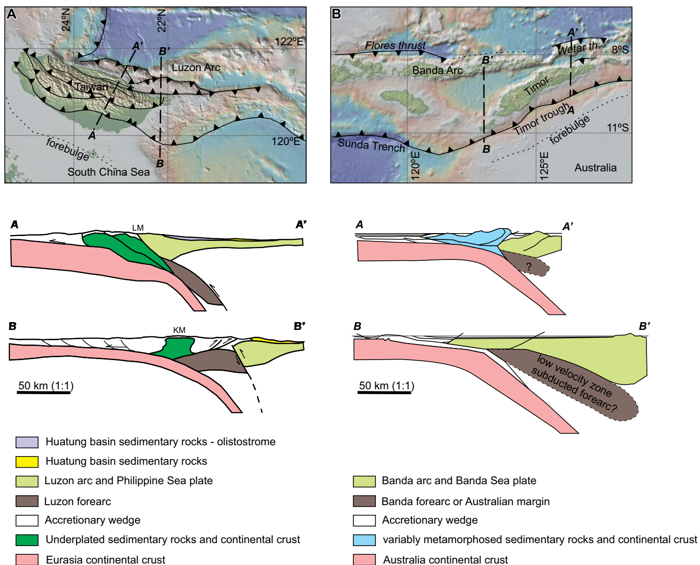
Figure 3. Maps and cross-sections showing the tectonic setting of (A) the China–Luzon arc (modified after McIntosh et al. 2005; LM – Lichi Mélange; KM – Kenting Mélange), and (B) Australia–Banda arc collisions (near surface simplified from Harris 2011, deep crust and mantle modified from Supendi et al. 2020). Background images and some plate boundaries were generated from www.geomapapp.org .
