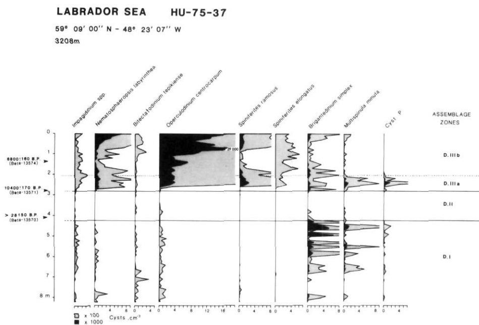
FIGURE 6. Dinocyst stratigraphy of core HU-75-37. Results are expressed in terms of concentrations.
