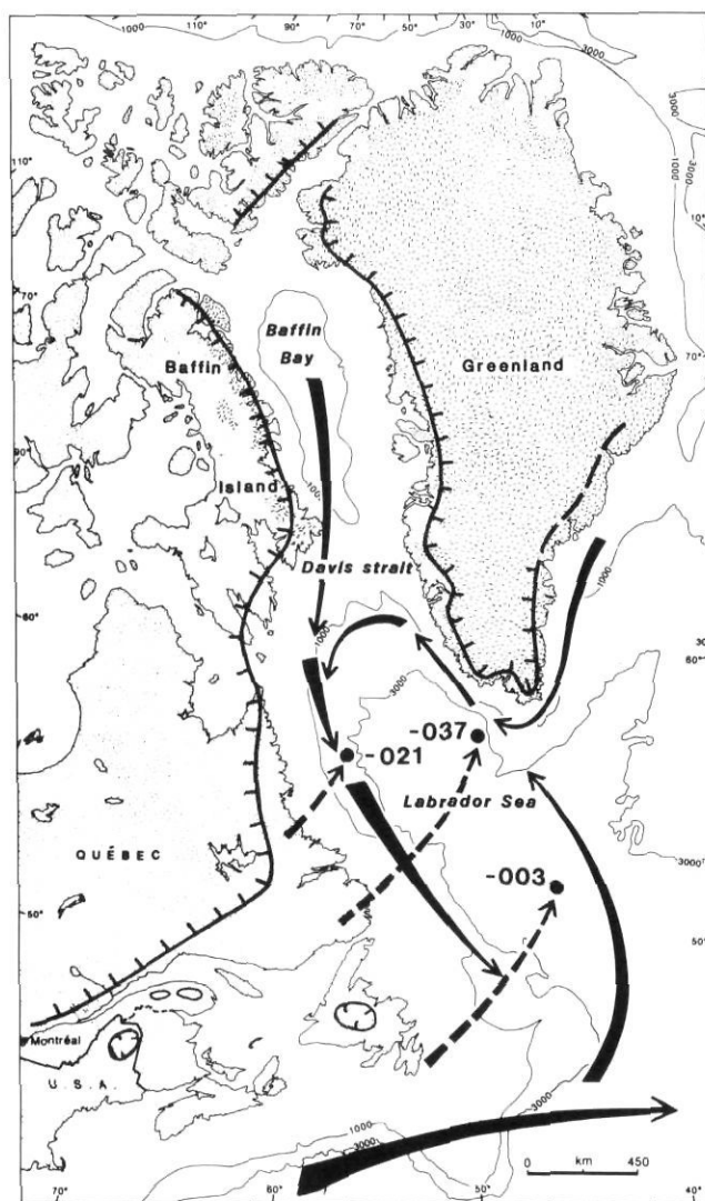
FIGURE 13. Schematic reconstruction of atmospheric (dashed arrows) and oceanic paleocirculations shortly after the deglaciation (after 11,000 BP). Probable ice limits ( \pi\pi ) are essentially based on PREST (1984).
