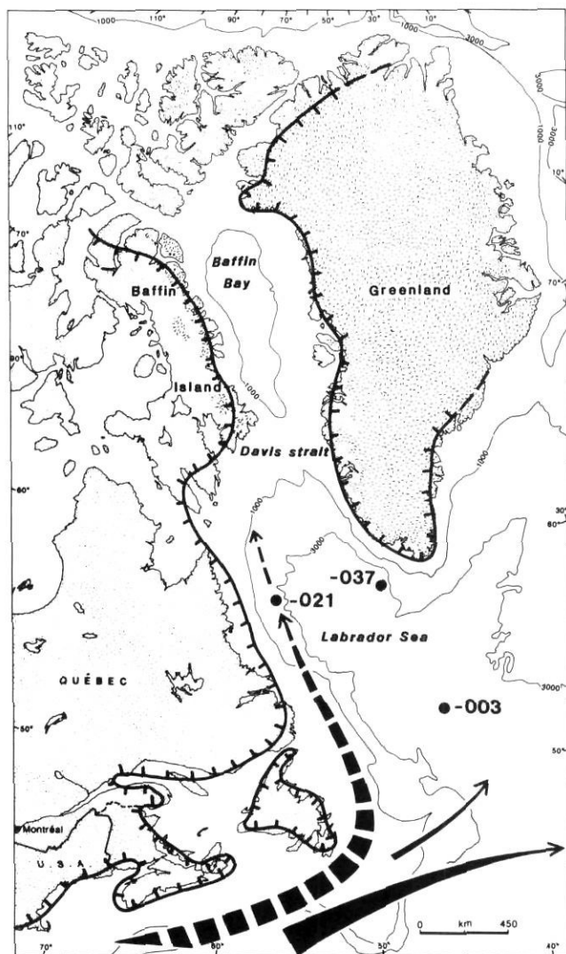
FIGURE 12. Schematic reconstruction of atmospheric (dashed arrows) and oceanic paleocirculation during the Late Wisconsinan (before 11,000 BP). Probable ice limits ( \pi\pi ) are based on a compilation of several studies (GRANT, 1977; ROGERSON, 1981; MILLER and DYKE, 1974; BOULTON, 1979; PREST, 1984; JOSEPHANS et al. , 1986).
