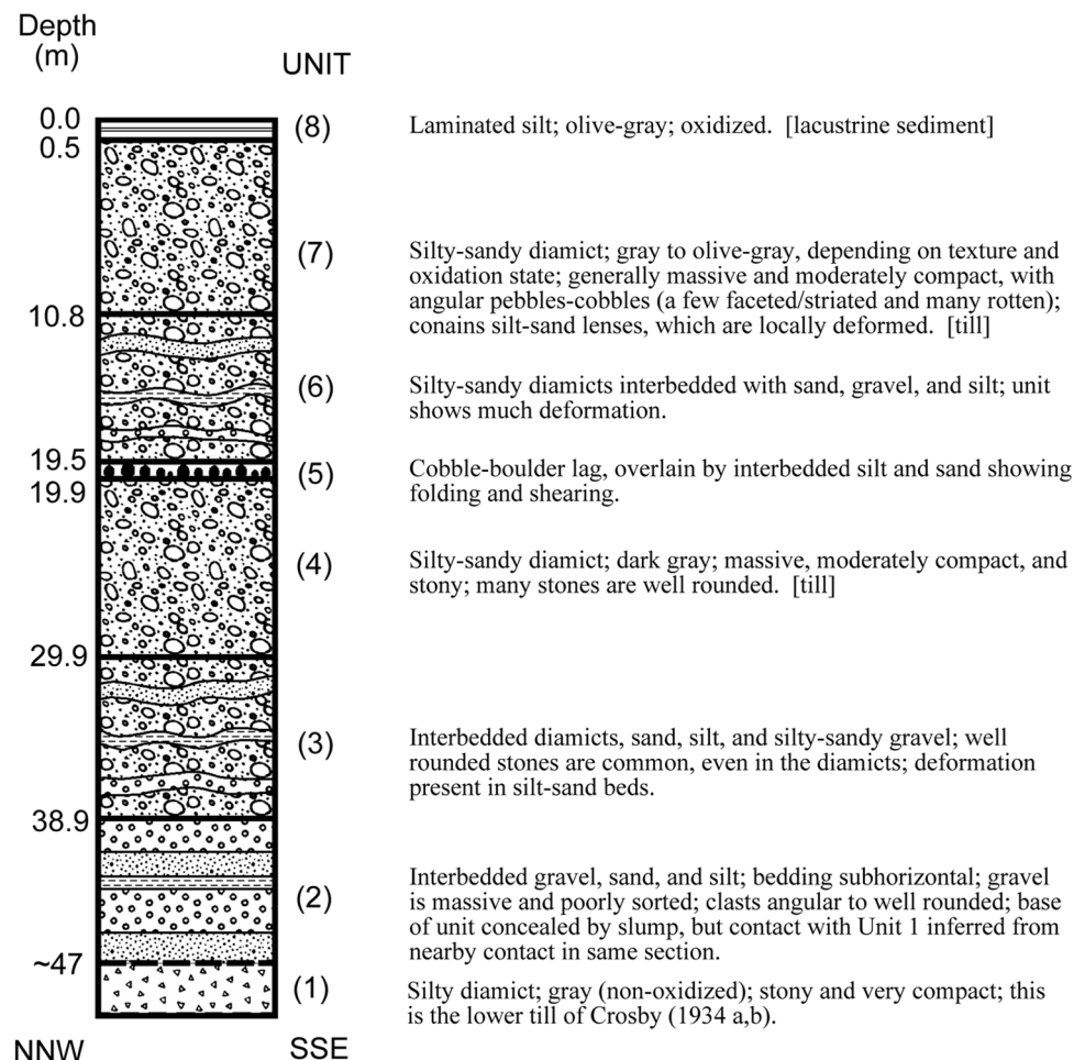
FIGURE 10. Stratigraphic log of Mill Brook section. Patterns within each unit schematically represent the range of sediment textures.
