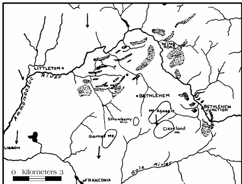
FIGURE 2. Part of map by J.W. Goldthwait (1916), showing inferred moraines (stippled areas) in Bethlehem, New Hampshire. Arrows indicate ice-flow direction at striation localities.
